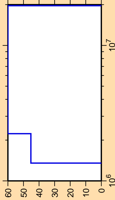
\Delta\sigma/\sigma vs. E for ^{162}\text{Hf}(n,n\alpha)
