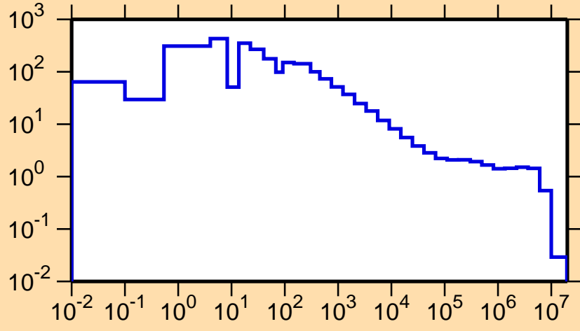
\sigma vs. E for ^{162}\text{Hf}(n,\gamma)
