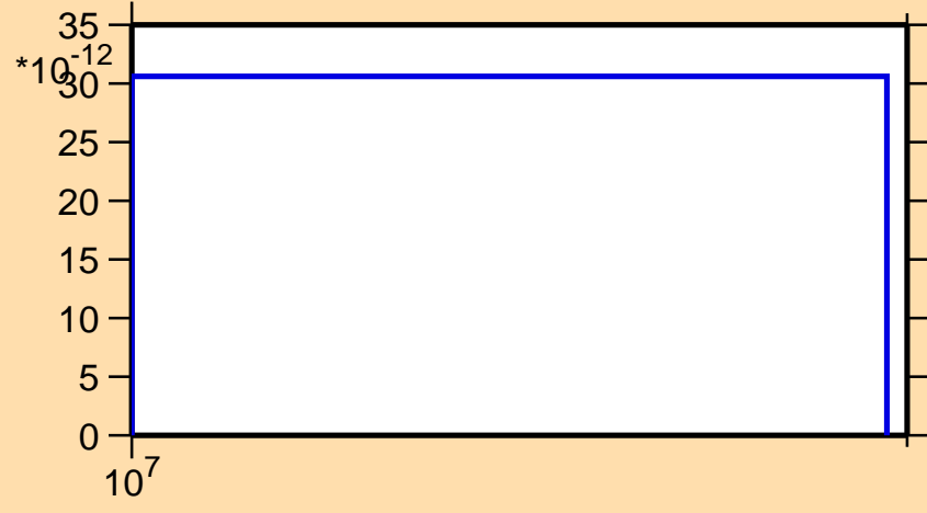
\sigma vs. E for ^{162}\text{Hf}(n,\text{pt})
