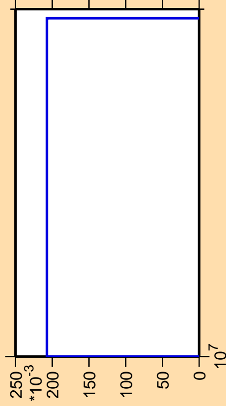
\Delta\sigma/\sigma vs. E for ^{162}\text{Hf}(n,nt)
