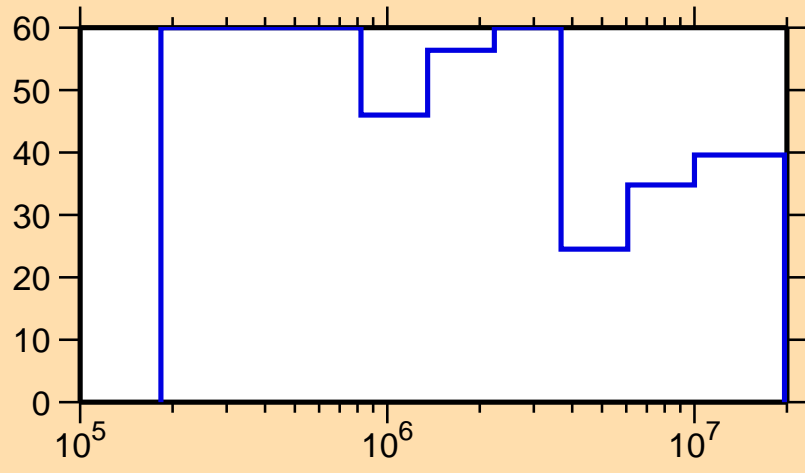
\Delta\sigma/\sigma vs. E for ^{162}\text{Hf}(n,\text{inel.})
