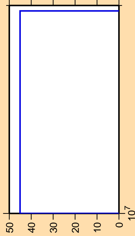
\Delta\sigma/\sigma vs. E for ^{162}\text{Hf}(n,n_1)
