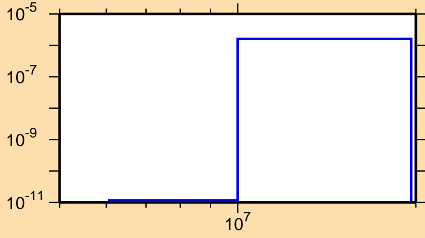
\sigma vs. E for ^{162}\text{Hf}(n,\text{He3})
