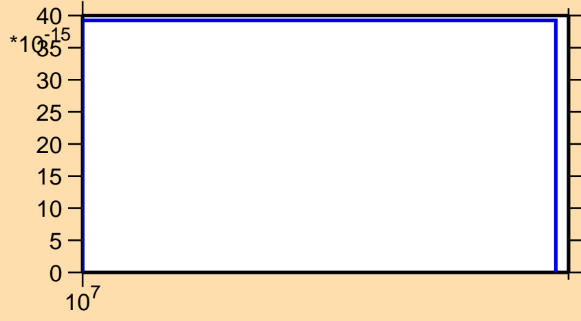
\sigma vs. E for ^{162}\text{Hf}(n,nt)
