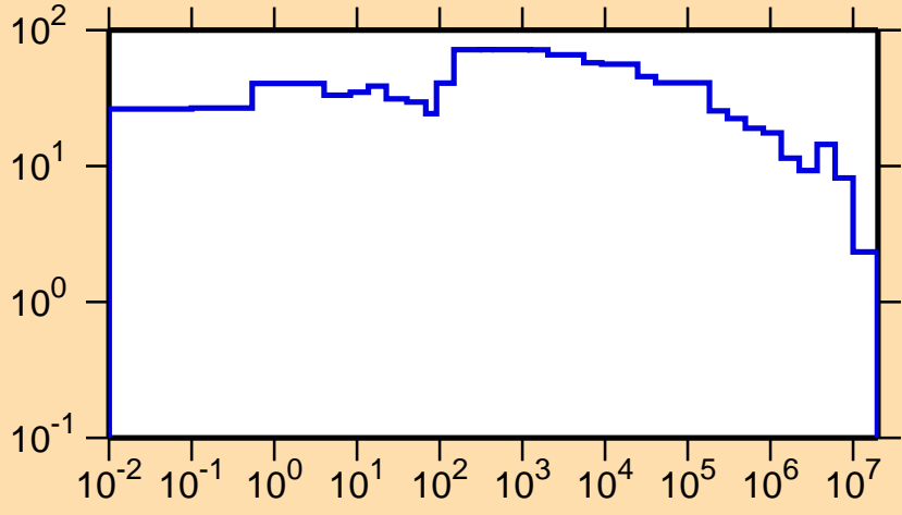
\Delta\sigma/\sigma vs. E for ^{162}\text{Hf}(n,\text{tot.})
