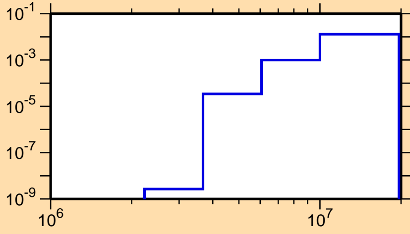
\sigma vs. E for ^{162}\text{Hf}(n,n\alpha)
