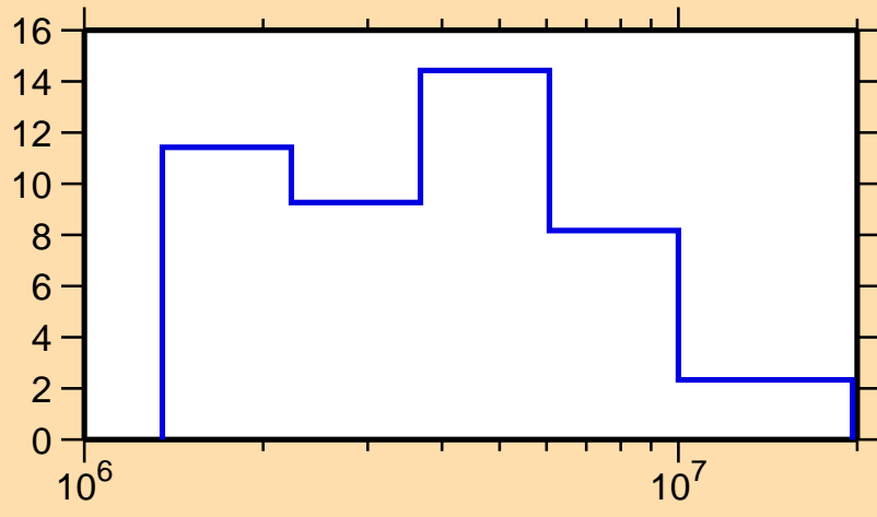
\Delta\sigma/\sigma vs. E for ^{162}\text{Hf}(n,\text{tot.})
