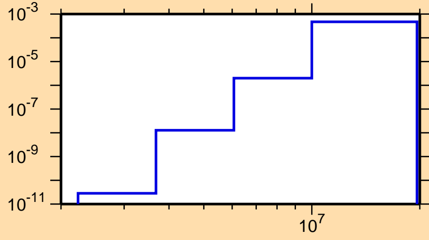
\sigma vs. E for ^{162}\text{Hf}(n,p\alpha)
