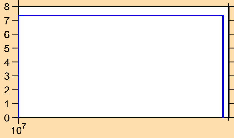
\Delta\sigma/\sigma vs. E for ^{162}\text{Hf}(n,\text{nonel.})
