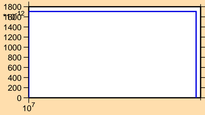
\sigma vs. E for ^{162}\text{Hf}(n,3n)
