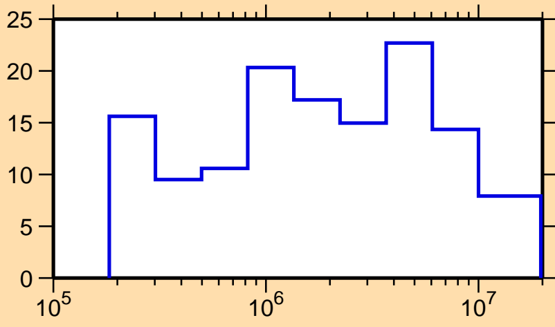
\Delta\sigma/\sigma vs. E for ^{162}\text{Hf}(n,\text{el.})
