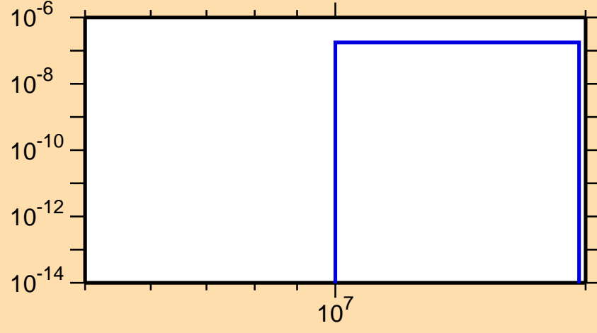
\sigma vs. E for ^{162}\text{Hf}(n,2n\alpha)
