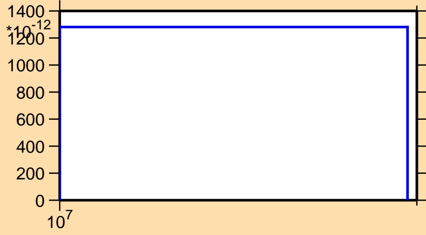
\sigma vs. E for ^{162}\text{Hf}(n,\text{nd})
