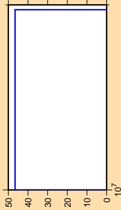
\Delta\sigma/\sigma vs. E for ^{162}\text{Hf}(n,n\text{cont.})
