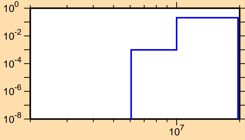
\sigma vs. E for ^{162}\text{Hf}(n,np)
