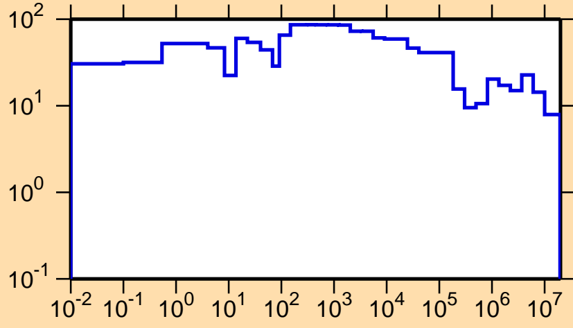
\Delta\sigma/\sigma vs. E for ^{162}\text{Hf}(n,\text{el.})
