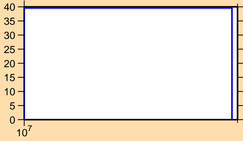
\Delta\sigma/\sigma vs. E for ^{162}\text{Hf}(n,\text{inel.})
