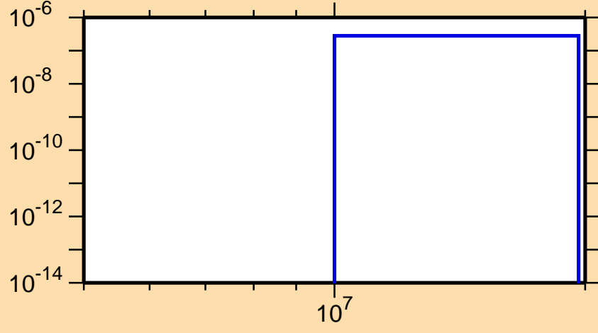
\sigma vs. E for ^{162}\text{Hf} (mt 45)
