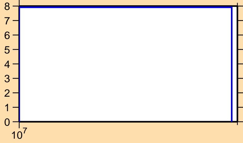
\Delta\sigma/\sigma vs. E for ^{162}\text{Hf}(n,\text{el.})
