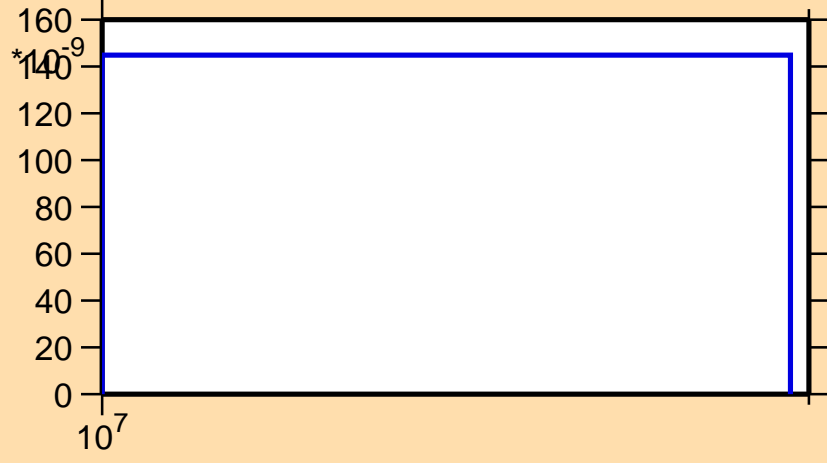
\sigma vs. E for ^{162}\text{Hf}(n,2np)
