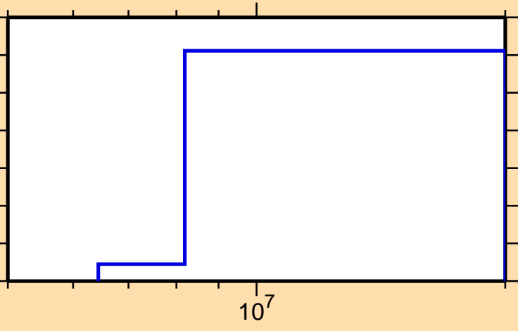
\sigma vs. E for ^{162}\text{Hf}(n,\text{He3})
