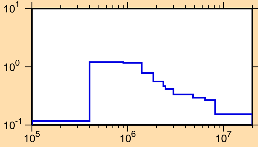
\sigma vs. E for ^{162}\text{Hf}(n,n_1)
