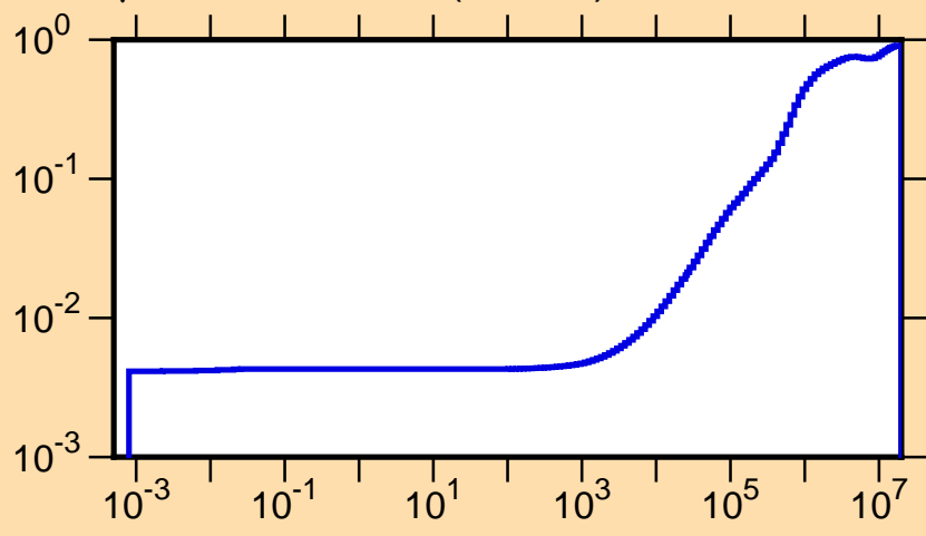
\mu vs. E for ^{163}\text{Hf(mt251)}
