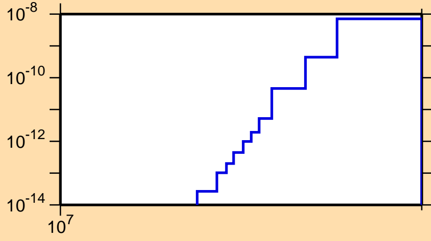
\sigma vs. E for ^{163}\text{Hf} (mt 34)
