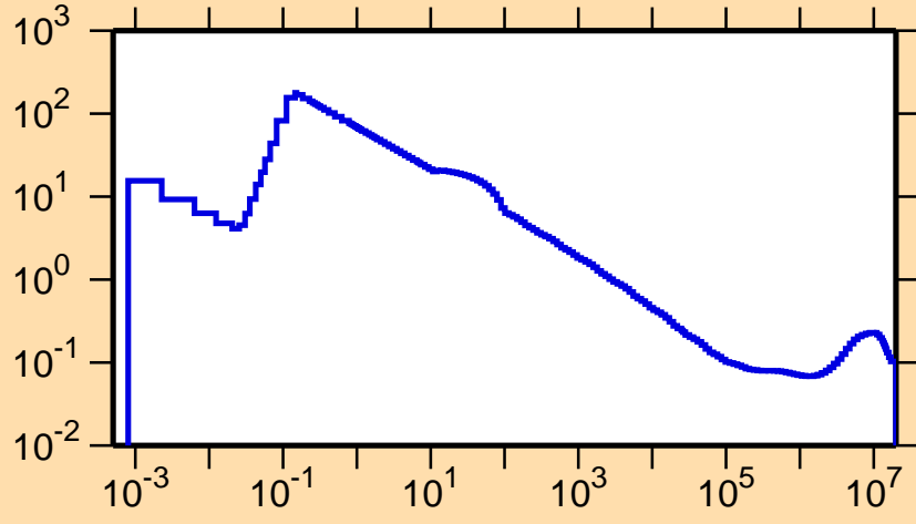
\sigma vs. E for ^{163}\text{Hf}(n,p)
