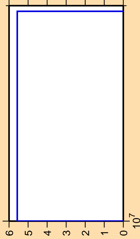
\Delta\sigma/\sigma vs. E for ^{163}\text{Hf}(n,nt)
