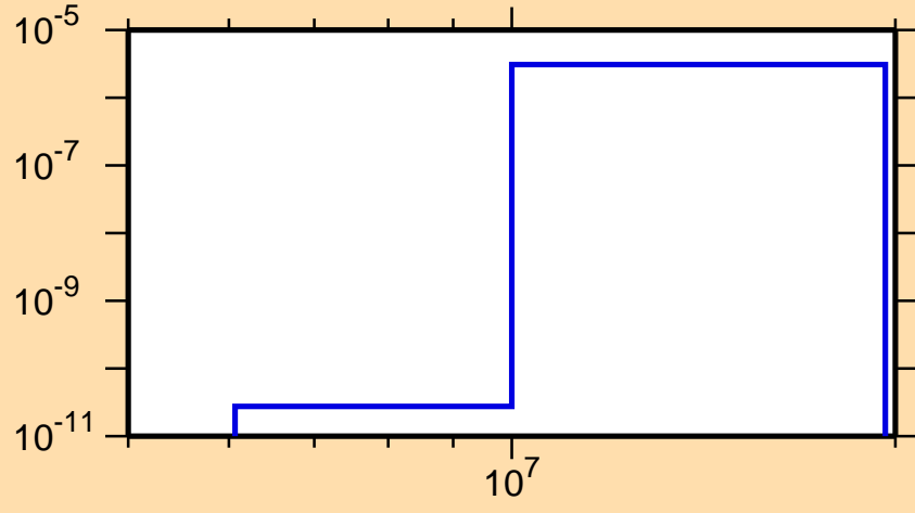
\sigma vs. E for ^{163}\text{Hf}(n,\text{He3})
