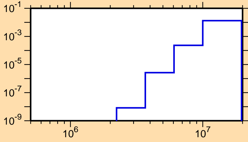
\sigma vs. E for ^{163}\text{Hf}(n,n\alpha)
