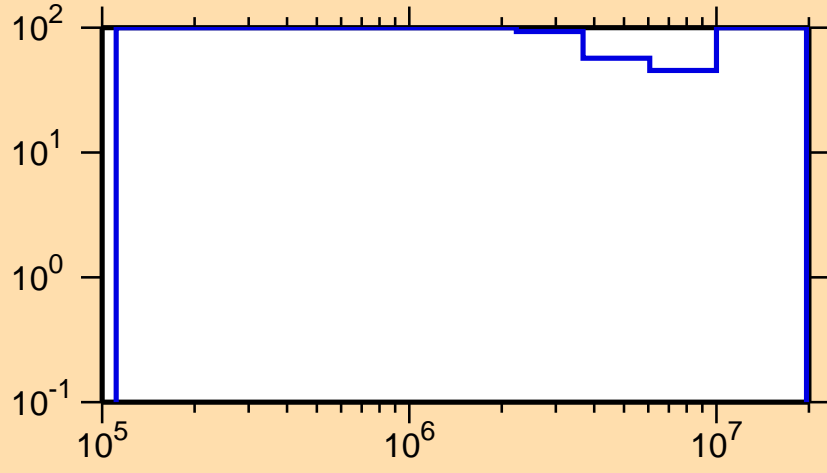
\Delta\sigma/\sigma vs. E for ^{163}\text{Hf}(n,n\text{cont.})
