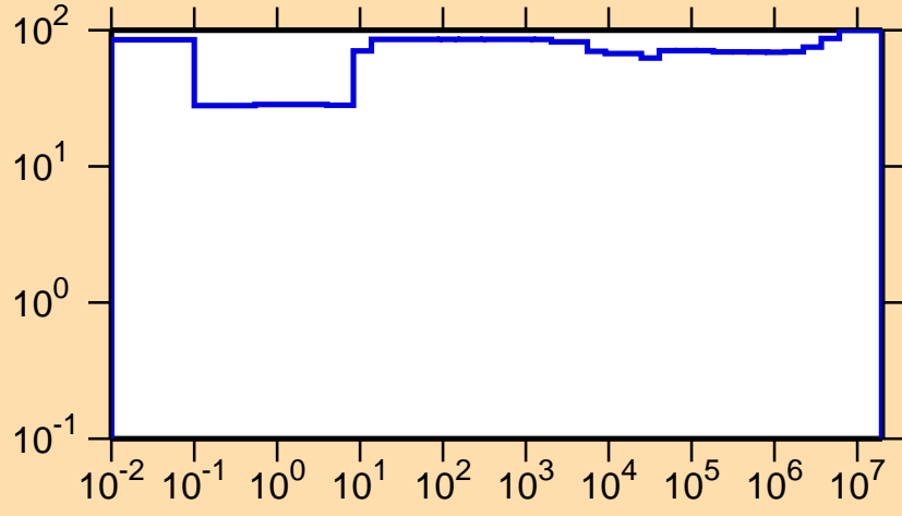
\Delta\sigma/\sigma vs. E for ^{163}\text{Hf}(n,\gamma)
