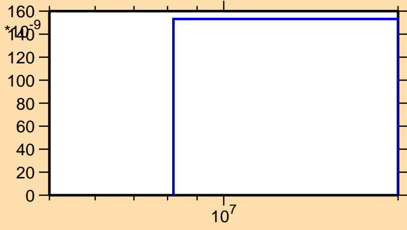
\sigma vs. E for ^{163}\text{Hf} (mt 45)
