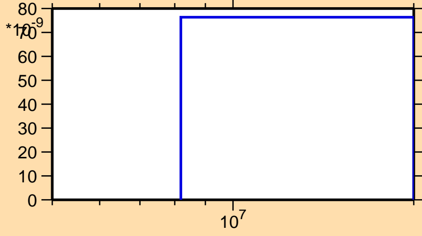
\sigma vs. E for ^{163}\text{Hf}(n,\text{pd})
