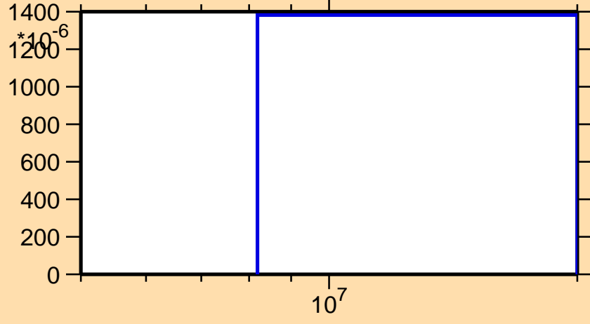
\sigma vs. E for ^{163}\text{Hf}(n,2n\alpha)
