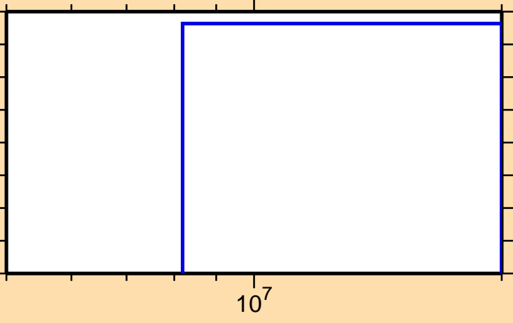
\sigma vs. E for ^{163}\text{Hf}(n,\text{pd})
