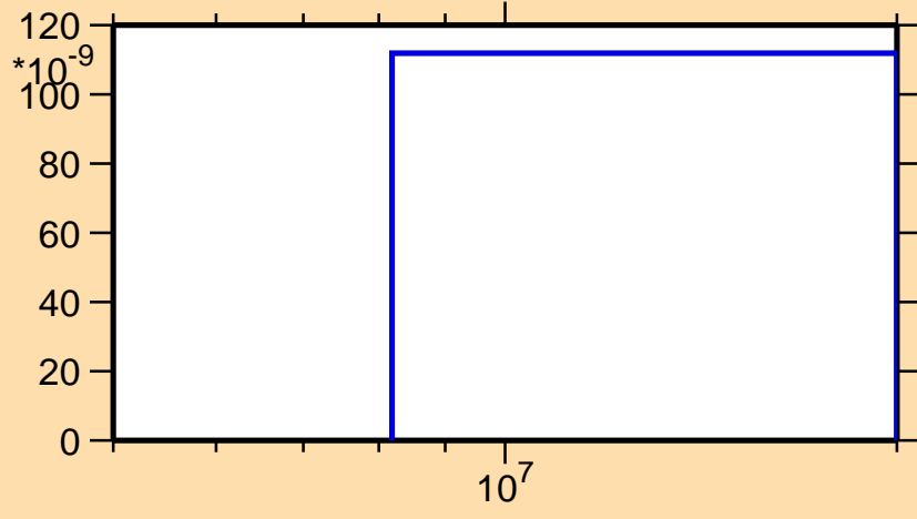
\sigma vs. E for ^{163}\text{Hf}(n,nd)
