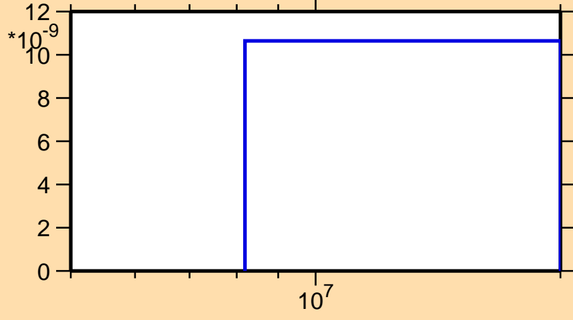
\sigma vs. E for ^{163}\text{Hf}(n,\text{pt})
