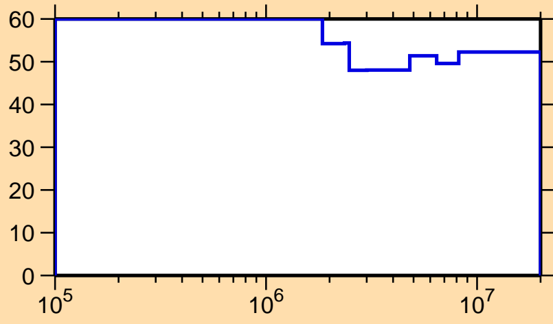
\Delta\sigma/\sigma vs. E for ^{163}\text{Hf}(n,n_1)
