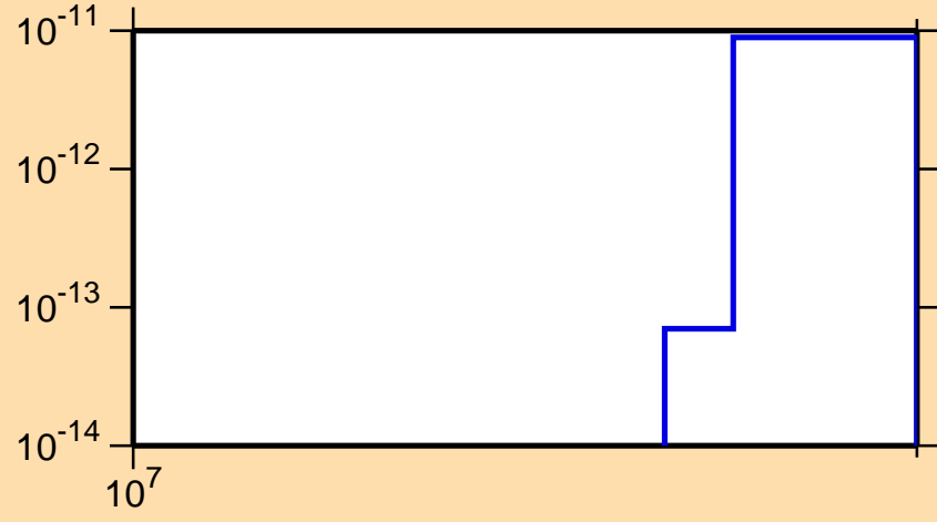
\sigma vs. E for ^{164}\text{Hf} (mt 34)
