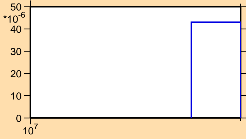
\sigma vs. E for ^{164}\text{Hf}(n,3n)
