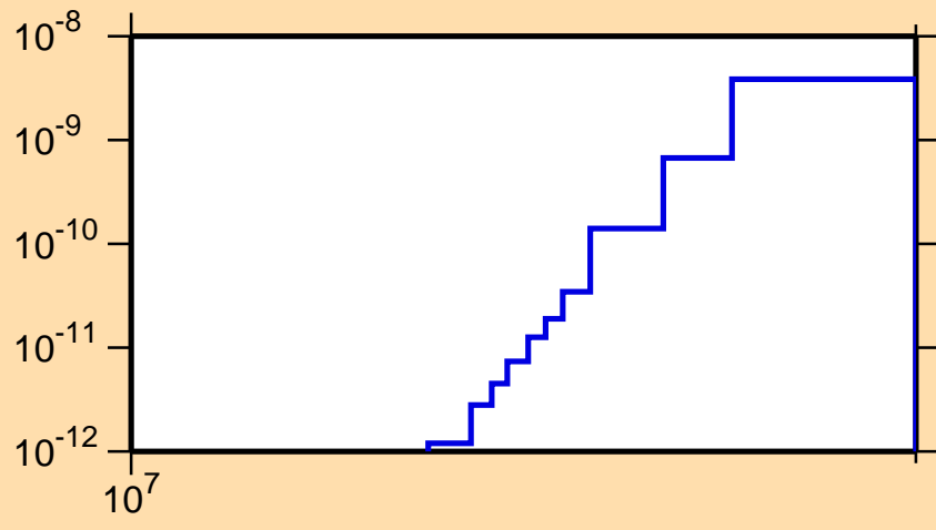
\sigma vs. E for ^{164}\text{Hf}(\text{mt117})
