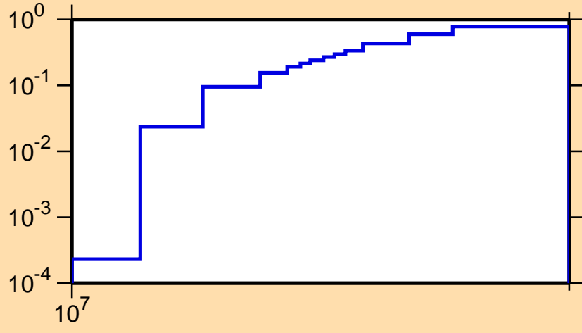
\sigma vs. E for ^{164}\text{Hf}(n,2n)
