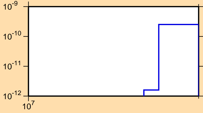
\sigma vs. E for ^{164}\text{Hf}(n,\text{pt})
