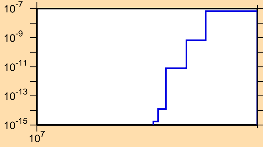
\sigma vs. E for ^{164}\text{Hf}(n,\text{nd})
