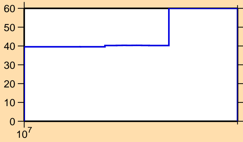
\Delta\sigma/\sigma vs. E for ^{164}\text{Hf}(n,\text{inel.})
