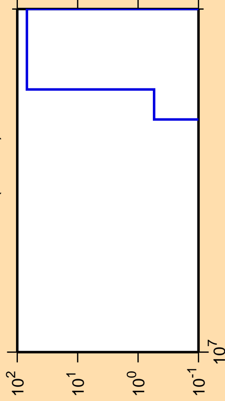
\Delta\sigma/\sigma vs. E for ^{164}\text{Hf} (mt 34)
