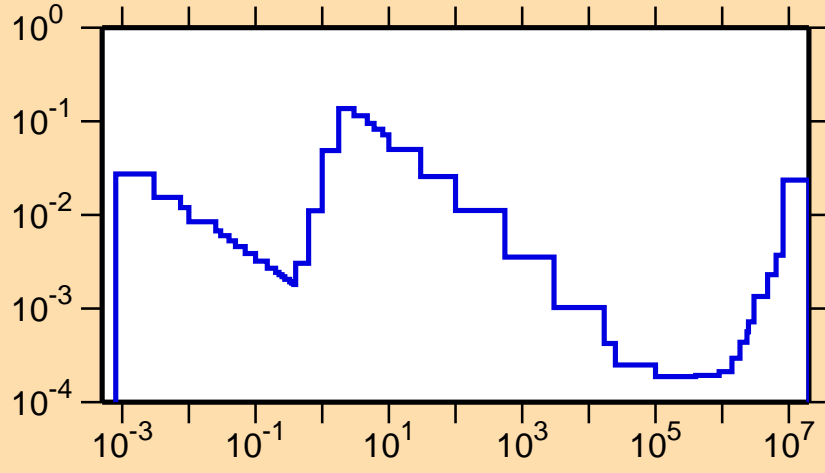
\sigma vs. E for ^{164}\text{Hf}(n,\alpha)
