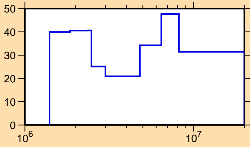
\Delta\sigma/\sigma vs. E for ^{164}\text{Hf}(n,el.)
