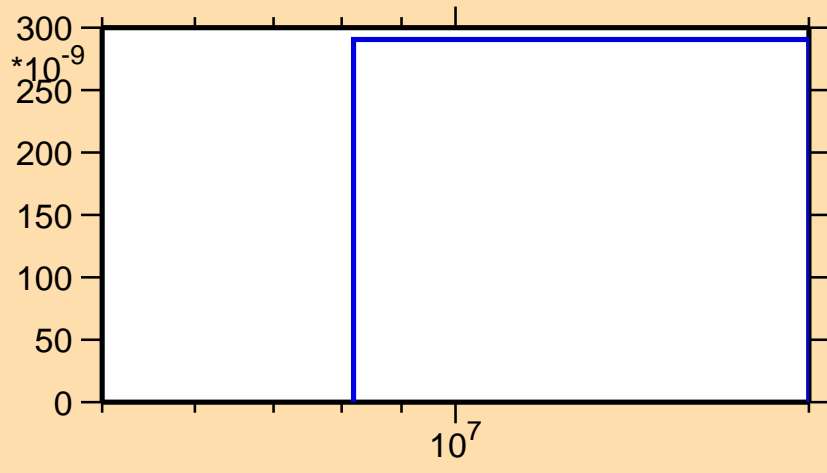
\sigma vs. E for ^{164}\text{Hf}(n,\text{He3})
