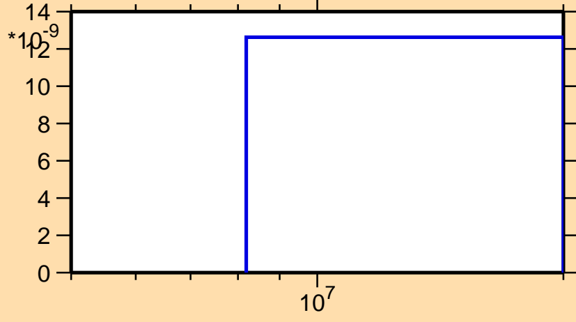
\sigma vs. E for ^{164}\text{Hf}(\text{mt } 45)
