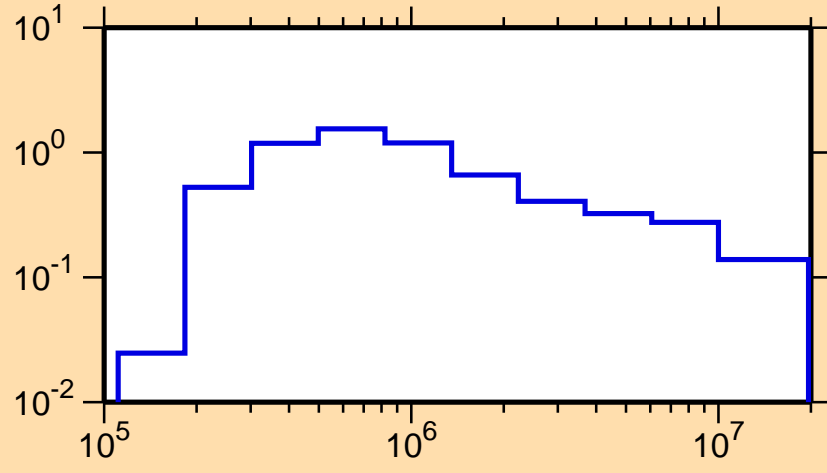
\sigma vs. E for ^{166}\text{Hf}(n,n_1)
