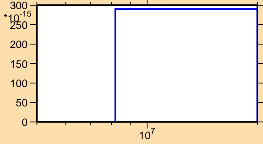
\sigma vs. E for ^{166}\text{Hf}(n,pt)
