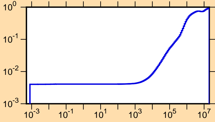
\mu vs. E for ^{168}\text{Hf(mt251)}
