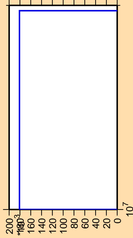
\Delta\sigma/\sigma vs. E for ^{168}\text{Hf}(n,\text{pt})
