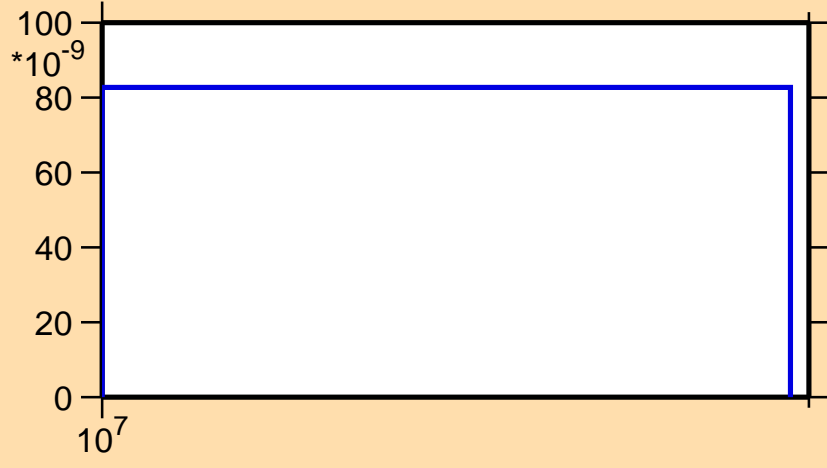
\sigma vs. E for ^{168}\text{Hf}(n,2n\alpha)
