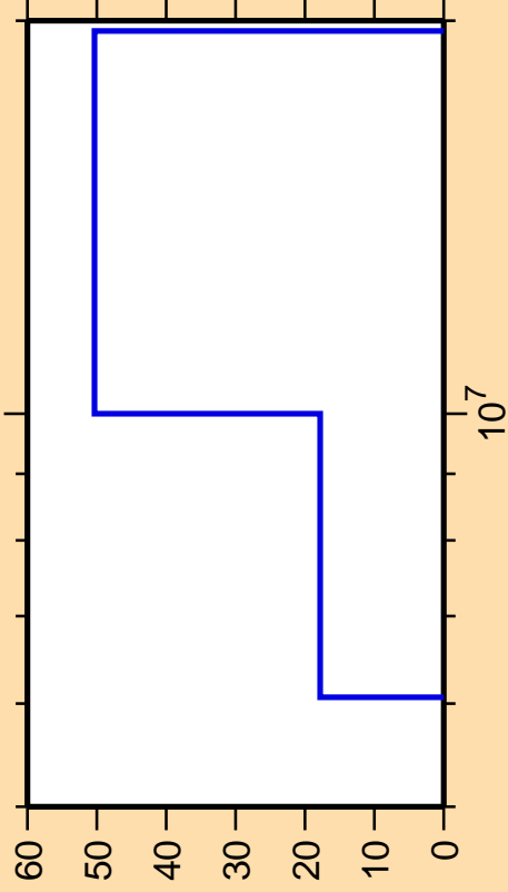
\Delta\sigma/\sigma vs. E for ^{168}\text{Hf}(n,p\alpha)
