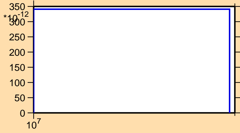
\sigma vs. E for ^{168}\text{Hf}(n,\text{nd})
