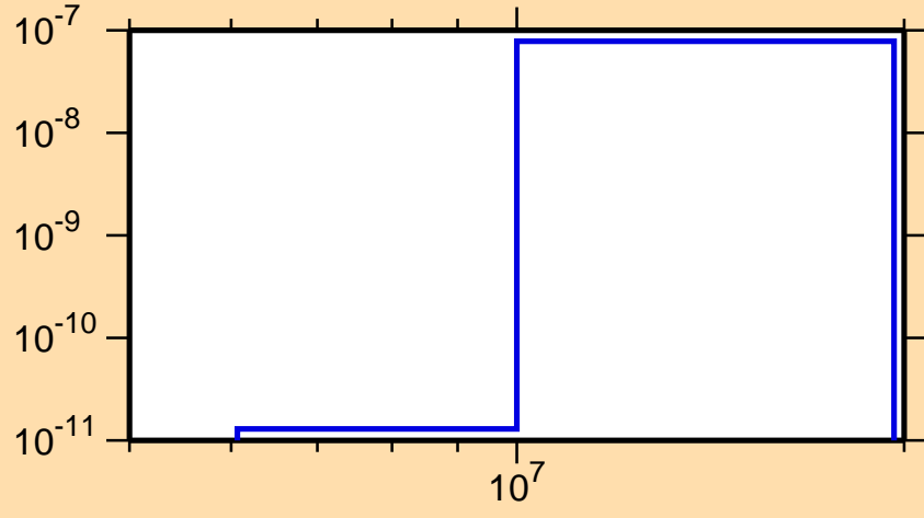
\sigma vs. E for ^{168}\text{Hf}(n,p\alpha)
