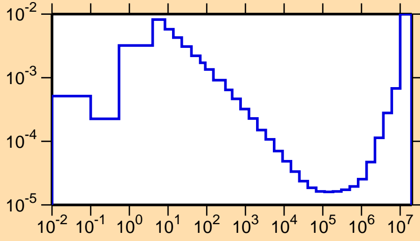
\sigma vs. E for ^{168}\text{Hf}(n,\alpha)
