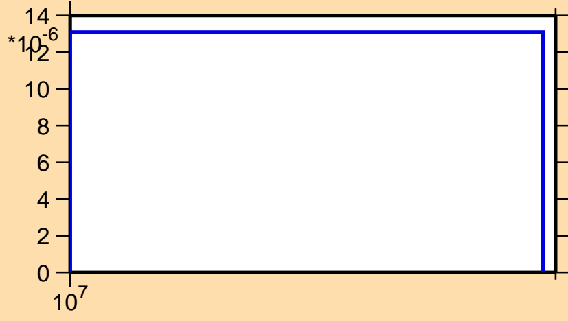
\sigma vs. E for ^{168}\text{Hf}(n,3n)
