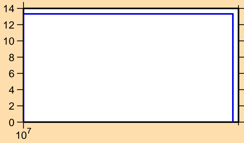
\Delta\sigma/\sigma vs. E for ^{168}\text{Hf}(n,\text{nonel.})
