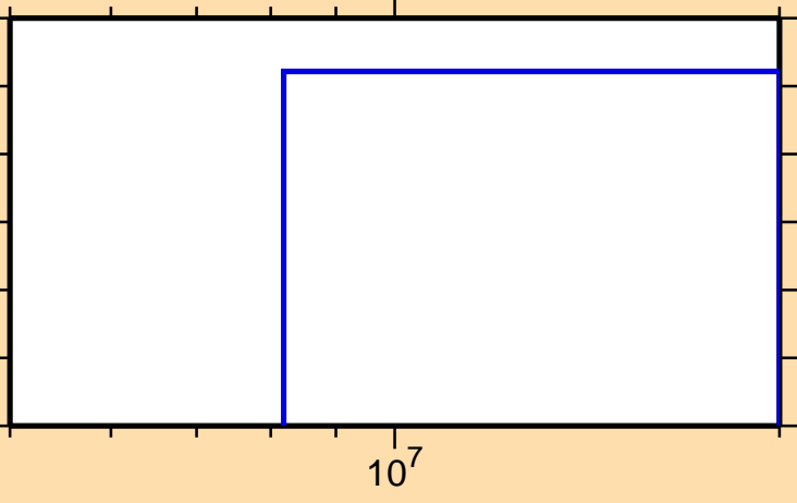
\sigma vs. E for ^{168}\text{Hf}(n,2np)
