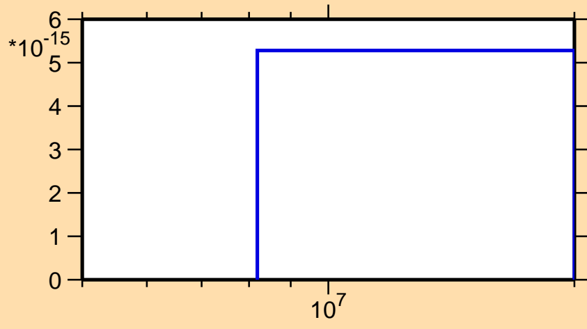
\sigma vs. E for ^{168}\text{Hf}(\text{mt } 34)
