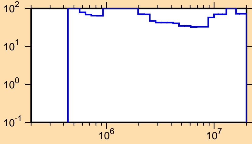
\Delta\sigma/\sigma vs. E for ^{169}\text{Hf}(n,n\text{cont.})
