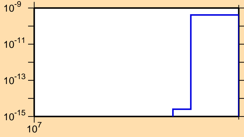
\sigma vs. E for ^{169}\text{Hf}(n,nt)
