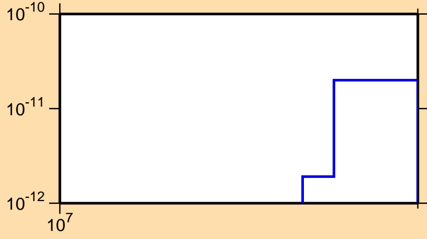
\sigma vs. E for ^{169}\text{Hf}(\text{mt117})
