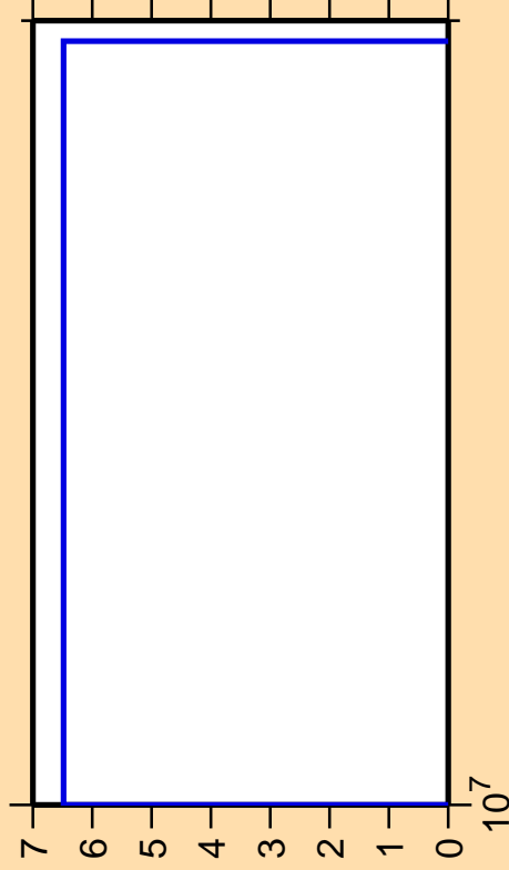
\Delta\sigma/\sigma vs. E for ^{169}\text{Hf} (mt 34)
