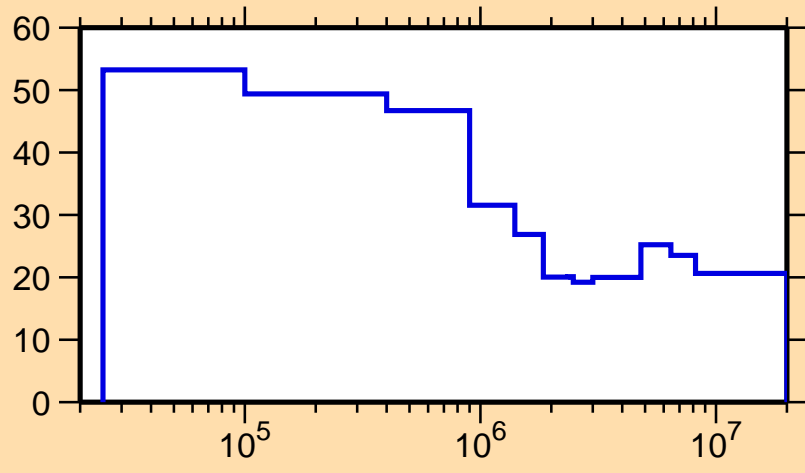
\Delta\sigma/\sigma vs. E for ^{169}\text{Hf}(n,\text{nonel.})
