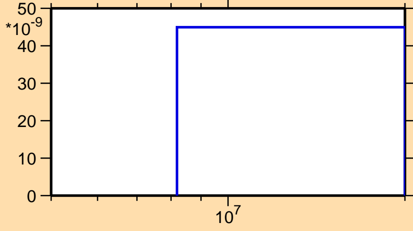
\sigma vs. E for ^{169}\text{Hf}(n,nd)
