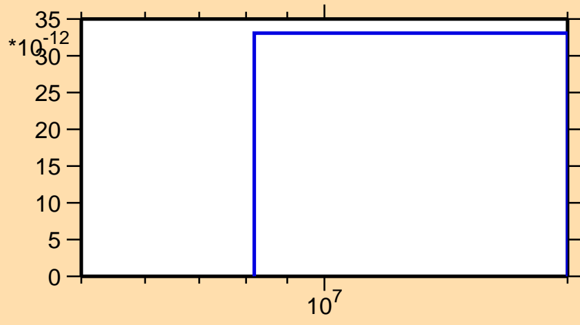
\sigma vs. E for ^{169}\text{Hf}(n,\text{pd})
