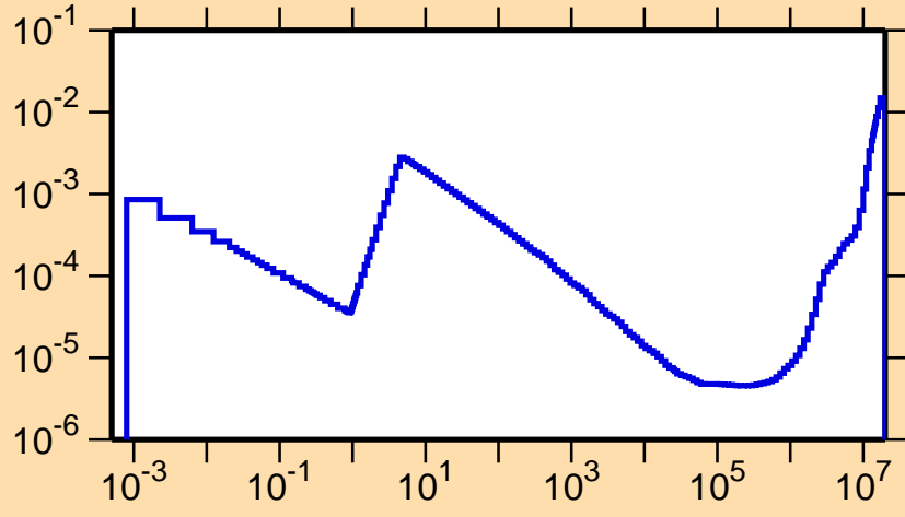
\sigma vs. E for ^{170}\text{Hf}(n,\alpha)
