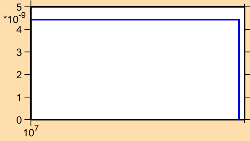
\sigma vs. E for ^{170}\text{Hf}(n,2np)
