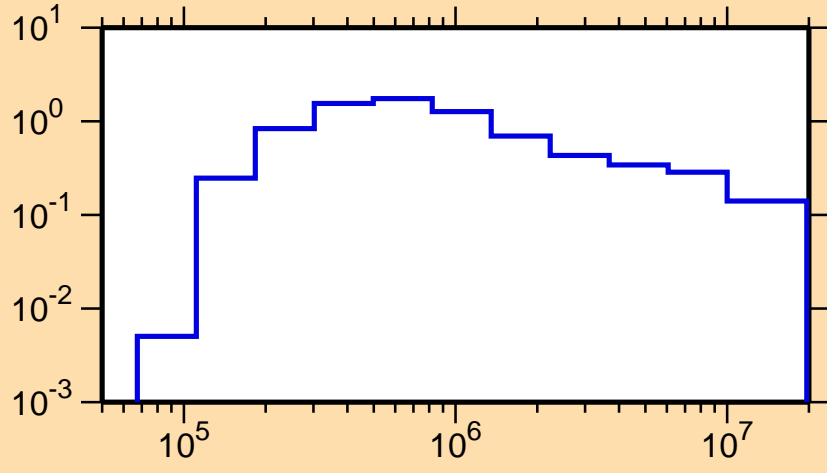
\sigma vs. E for ^{170}\text{Hf}(n,n_1)
