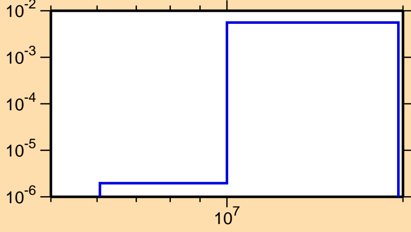
\sigma vs. E for ^{170}\text{Hf}(n,np)
