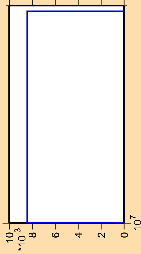
\Delta\sigma/\sigma vs. E for ^{170}\text{Hf} (mt 34)
