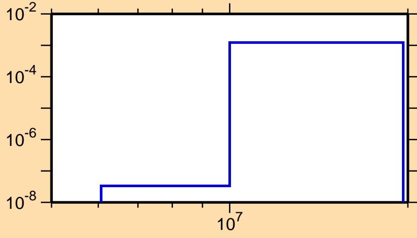
\sigma vs. E for ^{170}\text{Hf}(n,d)
