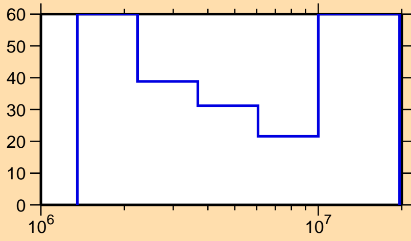
\Delta\sigma/\sigma vs. E for ^{170}\text{Hf}(n,n\text{cont.})
