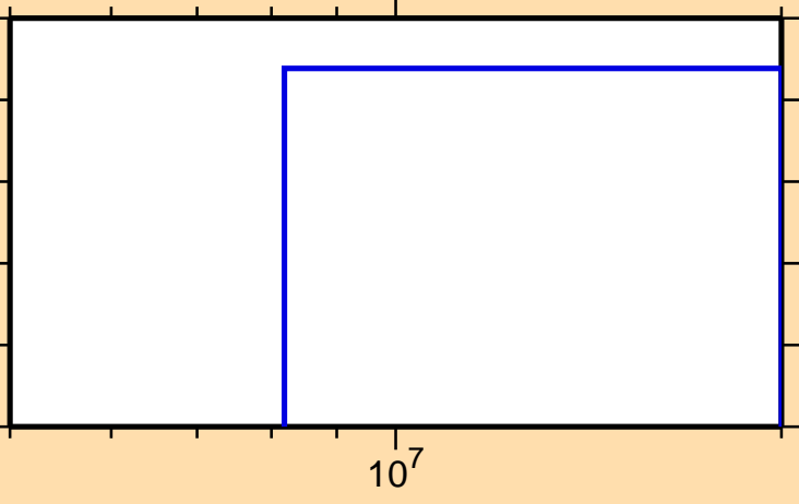
\sigma vs. E for ^{170}\text{Hf}(n,3n)
