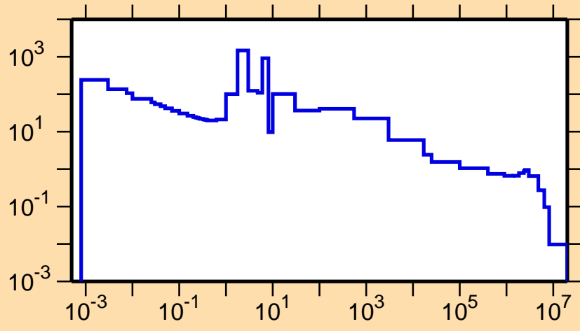
\sigma vs. E for ^{170}\text{Hf}(n,\gamma)
