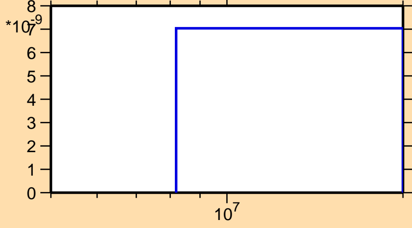
\sigma vs. E for ^{170}\text{Hf}(n,p\alpha)
