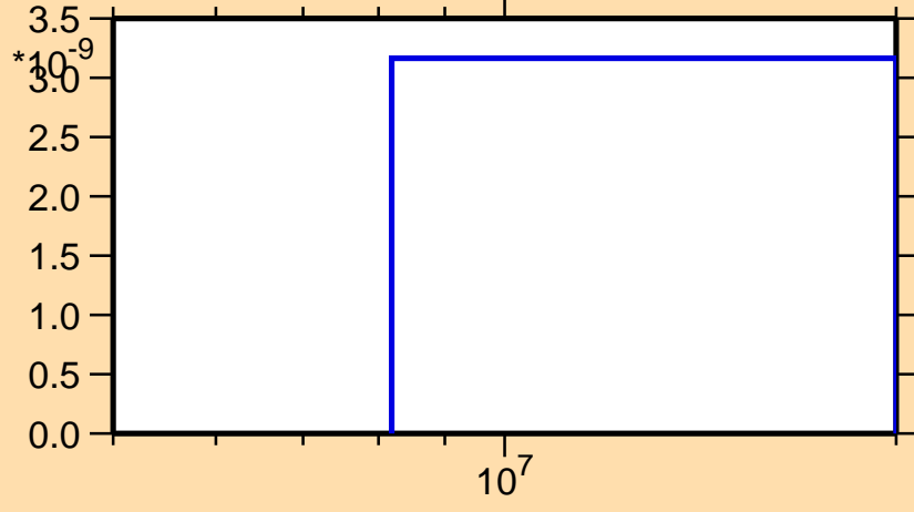
\sigma vs. E for ^{170}\text{Hf}(n,\text{He3})
