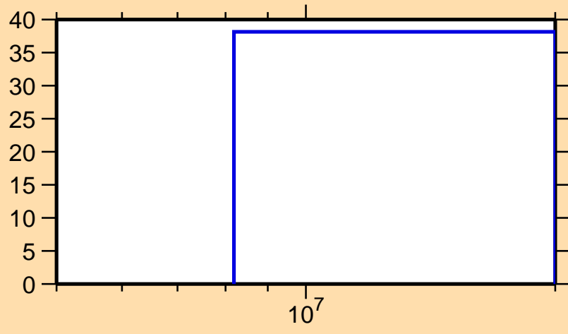
\Delta\sigma/\sigma vs. E for ^{170}\text{Hf}(n,2n)
