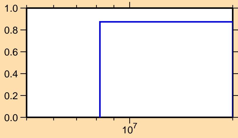
\sigma vs. E for ^{170}\text{Hf}(n,2n)
