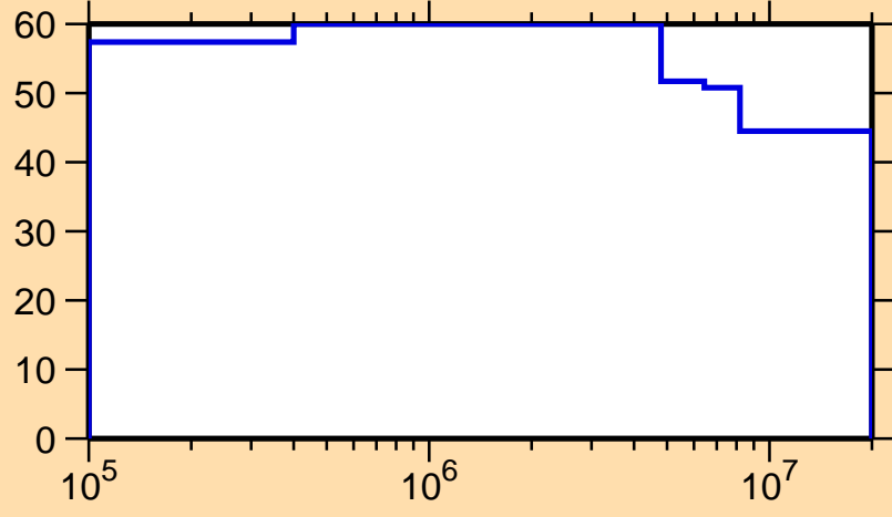
\Delta\sigma/\sigma vs. E for ^{170}\text{Hf}(n,n_1)
