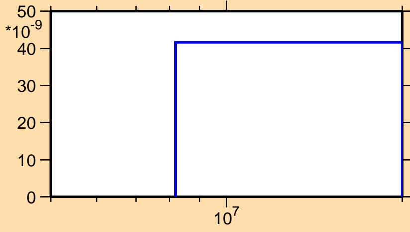
\sigma vs. E for ^{170}\text{Hf}(n,2n\alpha)
