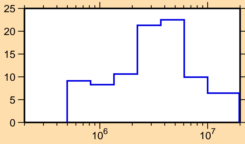
\Delta\sigma/\sigma vs. E for ^{171}\text{Hf}(n,el.)
