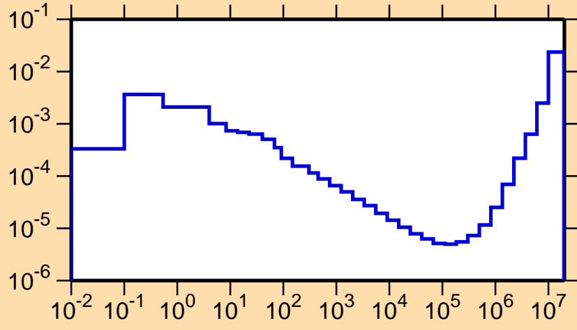
\sigma vs. E for ^{171}\text{Hf}(n,p)
