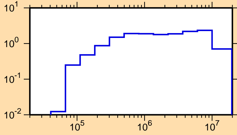
\sigma vs. E for ^{171}\text{Hf}(n,\text{inel.})
