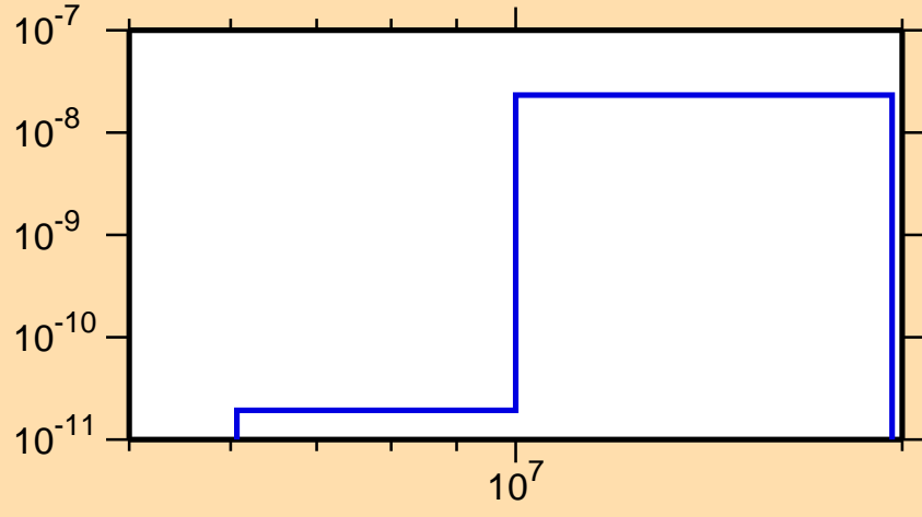
\sigma vs. E for ^{171}\text{Hf}(n,p\alpha)
