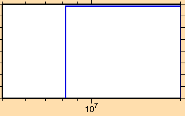
\sigma vs. E for ^{171}\text{Hf}(n,2n\alpha)
