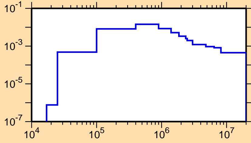
\sigma vs. E for ^{171}\text{Hf}(n,n_1)
