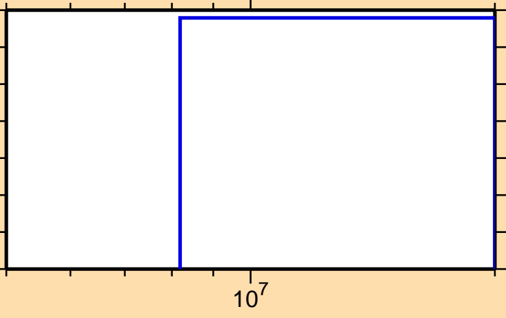
\sigma vs. E for ^{172}\text{Hf}(n,3n)
