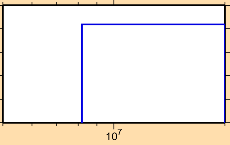
\sigma vs. E for ^{172}\text{Hf}(n,2n\alpha)
