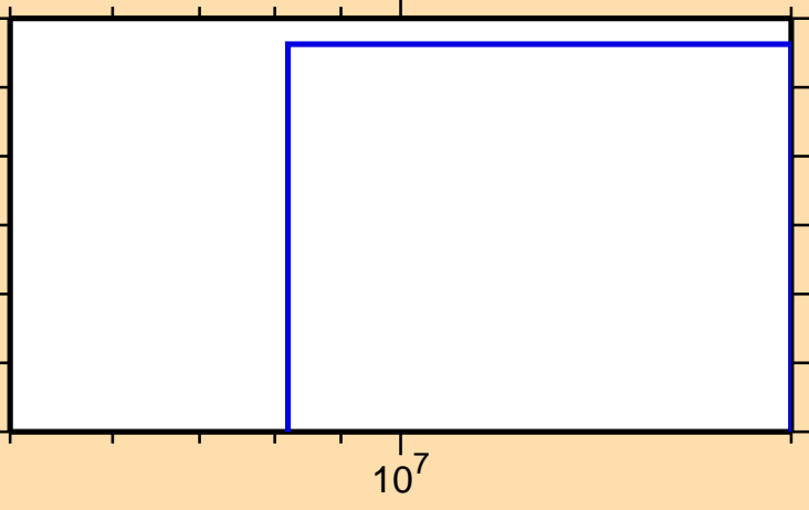
\sigma vs. E for ^{173}\text{Hf}(n,2n\alpha)
