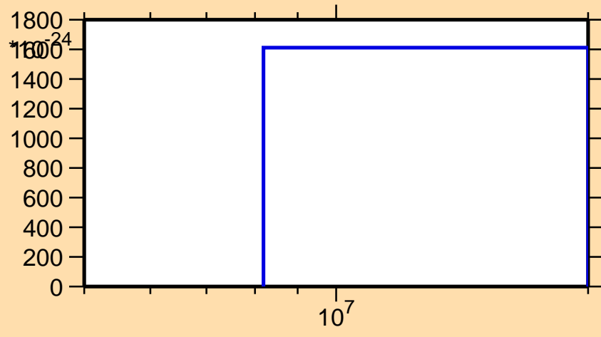
\sigma vs. E for ^{173}\text{Hf}(\text{mt } 11)
