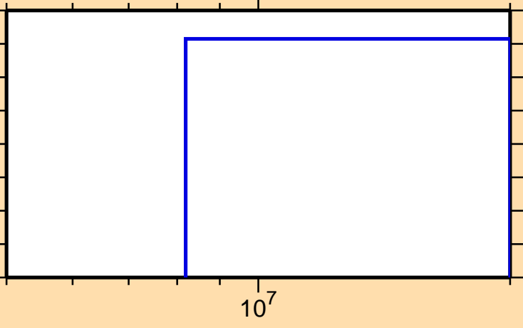
\sigma vs. E for ^{173}\text{Hf}(n,pd)
