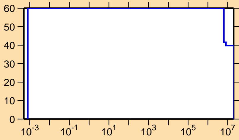
\Delta\sigma/\sigma vs. E for ^{173}\text{Hf}(n,p)
