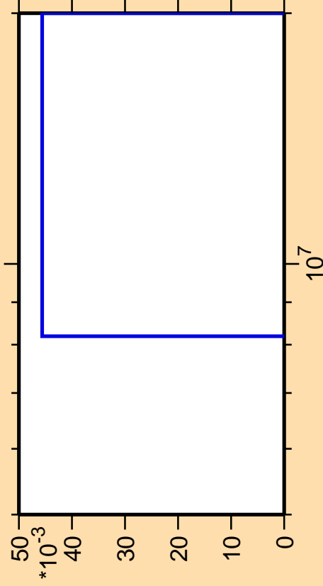
\Delta\sigma/\sigma vs. E for ^{173}\text{Hf}(n,pd)
