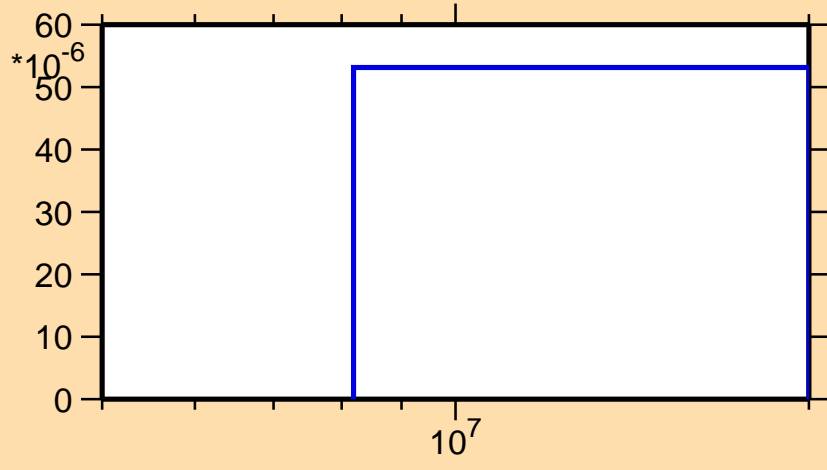
\sigma vs. E for ^{173}\text{Hf}(n,t)
