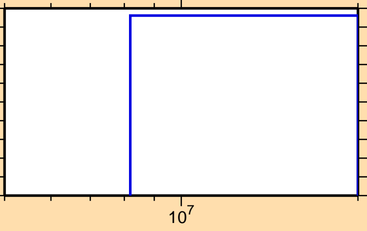
\sigma vs. E for ^{173}\text{Hf}(n,3n)
