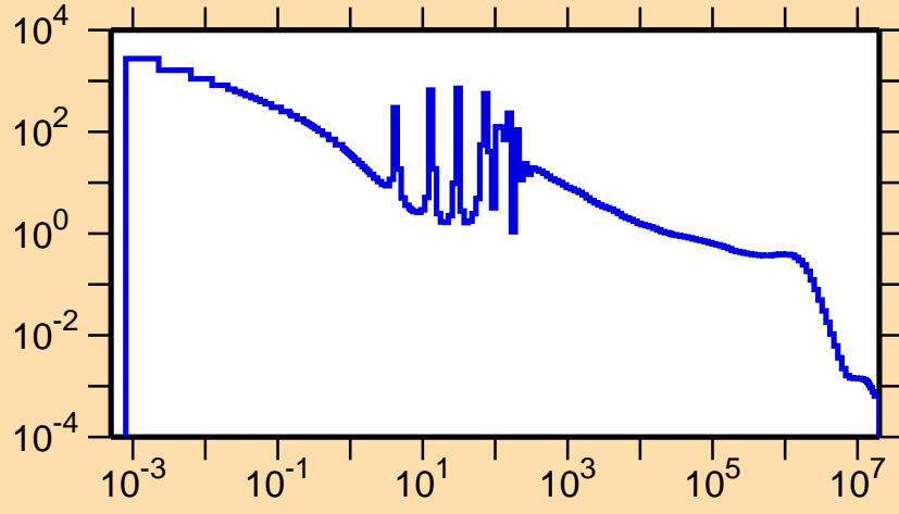
\sigma vs. E for ^{174}\text{Hf}(n,\gamma)
