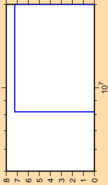
\Delta\sigma/\sigma vs. E for ^{174}\text{Hf}(n,2n)
