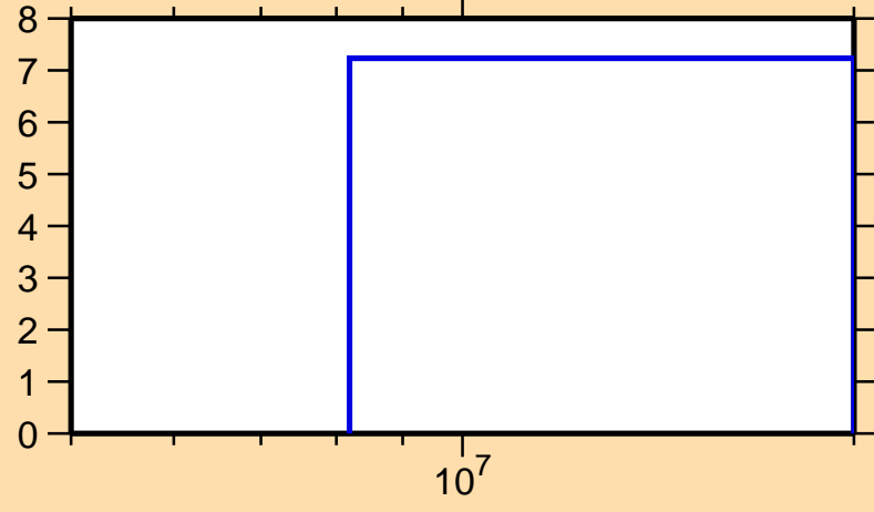
\Delta\sigma/\sigma vs. E for ^{174}\text{Hf}(n,2n)
