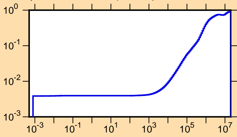
\mu vs. E for ^{175}\text{Hf}(\text{mt251})
