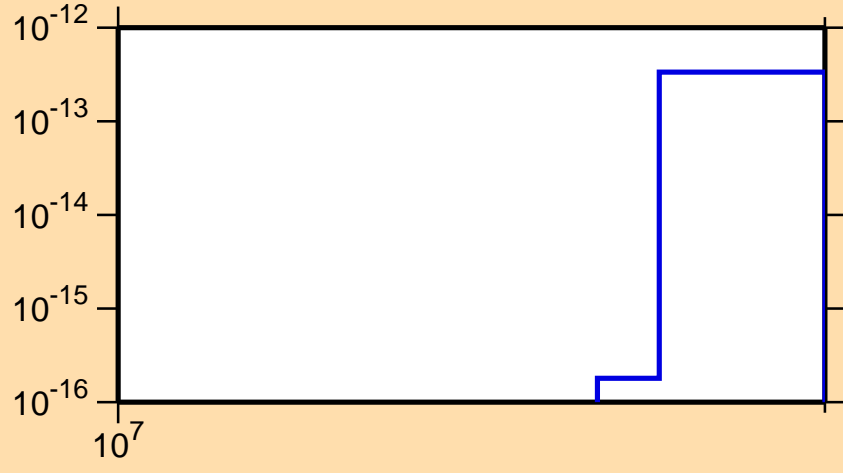
\sigma vs. E for ^{175}\text{Hf}(\text{mt } 34)
