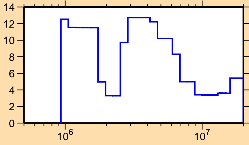
\Delta\sigma/\sigma vs. E for ^{175}\text{Hf}(n,\text{tot.})
