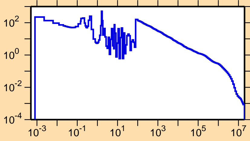
\sigma vs. E for ^{175}\text{Hf}(n,\gamma)
