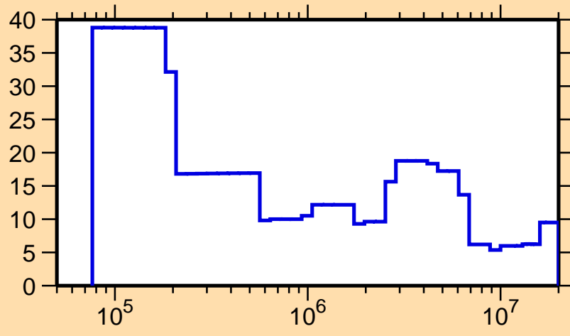
\Delta\sigma/\sigma vs. E for ^{175}\text{Hf}(n,\text{el.})
