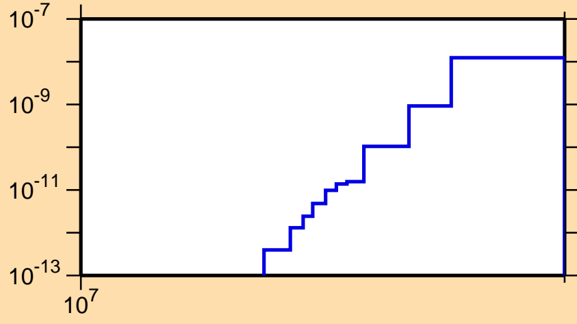
\sigma vs. E for ^{175}\text{Hf}(n,\text{He3})
