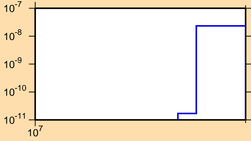
\sigma vs. E for ^{175}\text{Hf}(n,nt)
