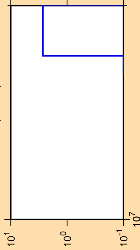
\Delta\sigma/\sigma vs. E for ^{175}\text{Hf}(\text{mt } 34)
