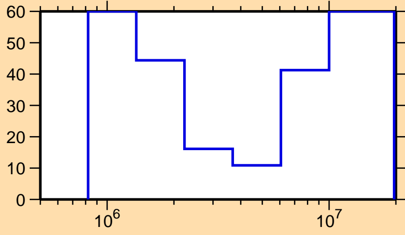
\Delta\sigma/\sigma vs. E for ^{175}\text{Hf}(n,n\text{cont.})
