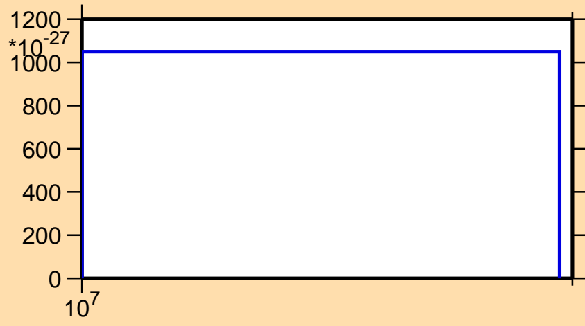
\sigma vs. E for ^{175}\text{Hf} (mt 11)
