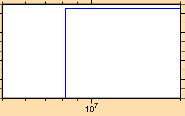
\sigma vs. E for ^{175}\text{Hf}(n,nt)
