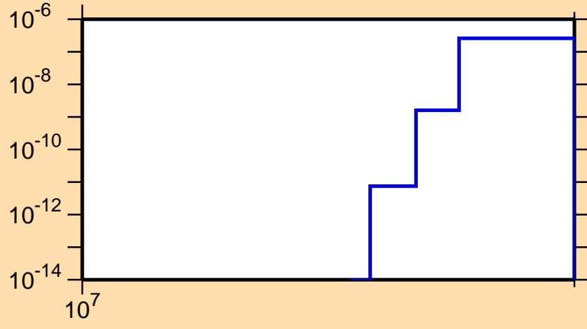
\sigma vs. E for ^{176}\text{Hf}(n,\text{nd})
