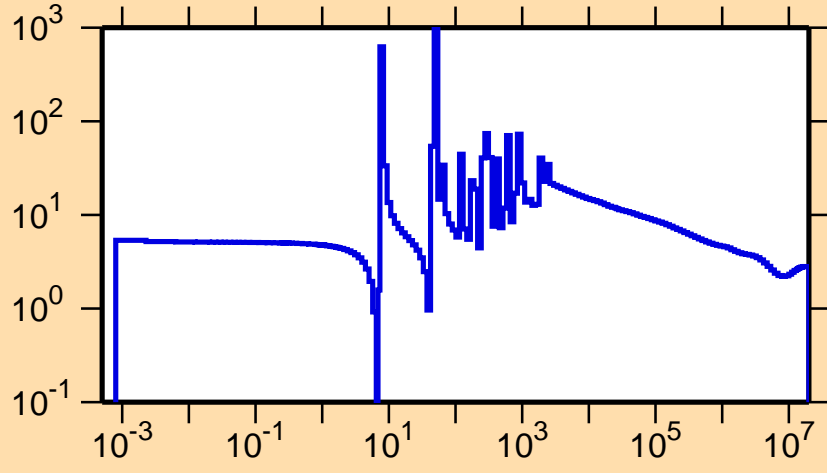
\sigma vs. E for ^{176}\text{Hf}(n,\text{el.})
