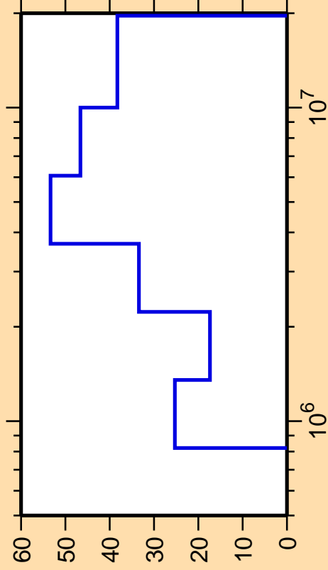
\Delta\sigma/\sigma vs. E for ^{176}\text{Hf}(n,n_4)
