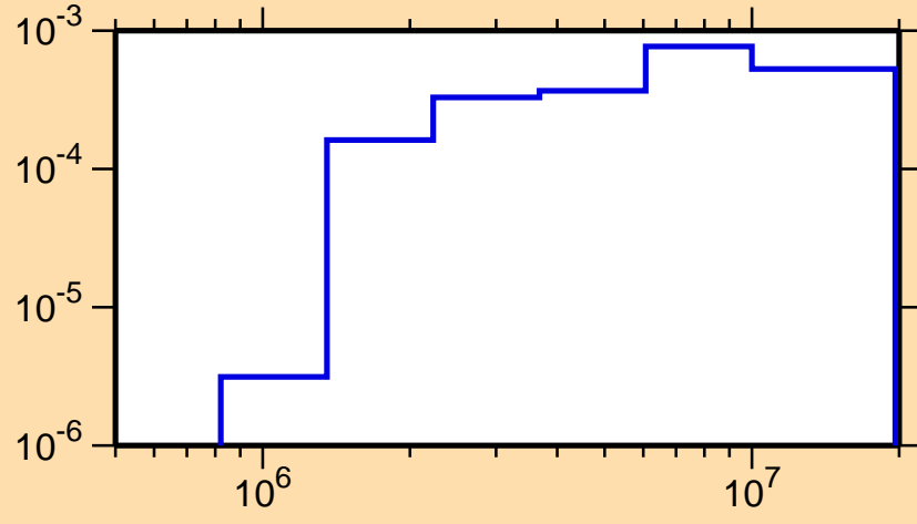
\sigma vs. E for ^{176}\text{Hf}(n,n_4)
