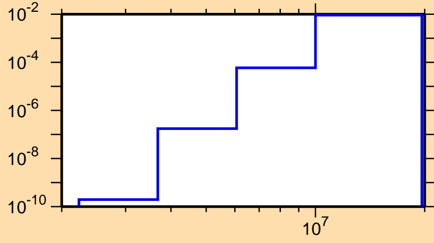
\sigma vs. E for ^{176}\text{Hf}(n,p)
