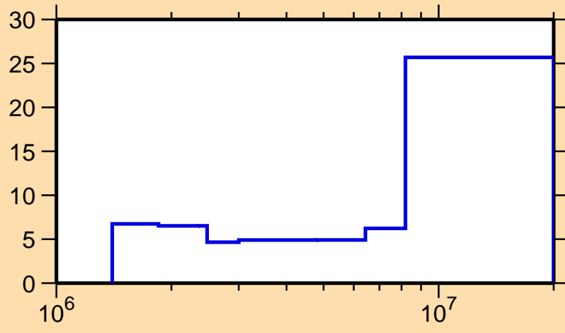
\Delta\sigma/\sigma vs. E for ^{176}\text{Hf}(n,n\text{cont.})
