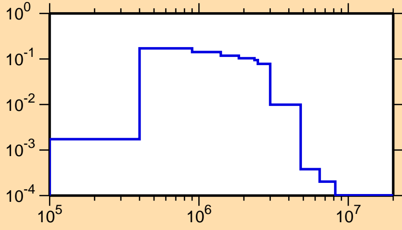
\sigma vs. E for ^{177}\text{Hf}(n,n_4)
