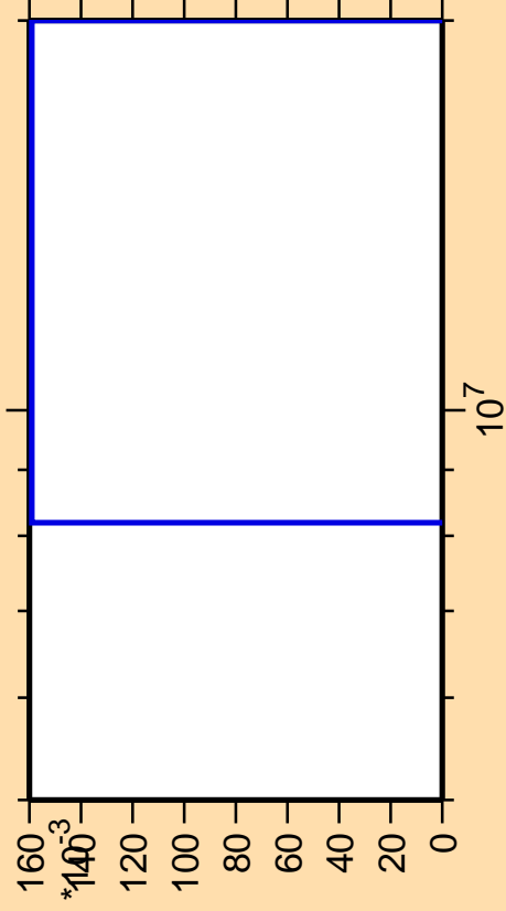
\Delta\sigma/\sigma vs. E for ^{177}\text{Hf}(n,p\alpha)
