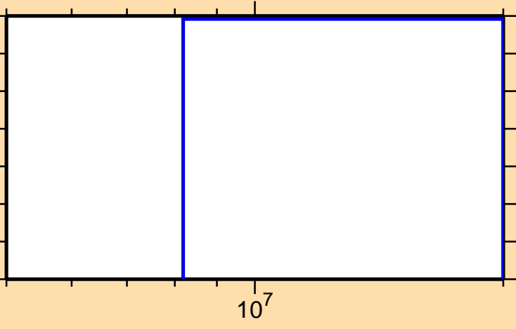
\sigma vs. E for ^{177}\text{Hf}(n,nt)
