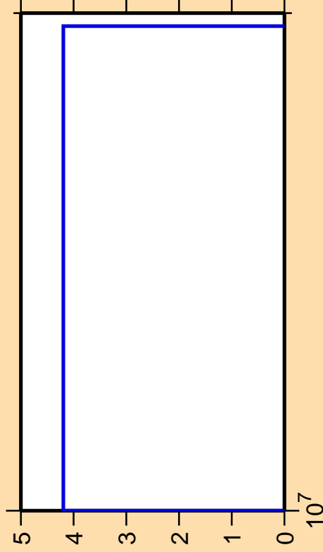
\Delta\sigma/\sigma vs. E for ^{177}\text{Hf}(n,3n\alpha)
