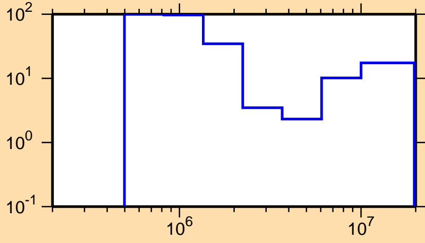
\Delta\sigma/\sigma vs. E for ^{177}\text{Hf}(n,ncont.)
