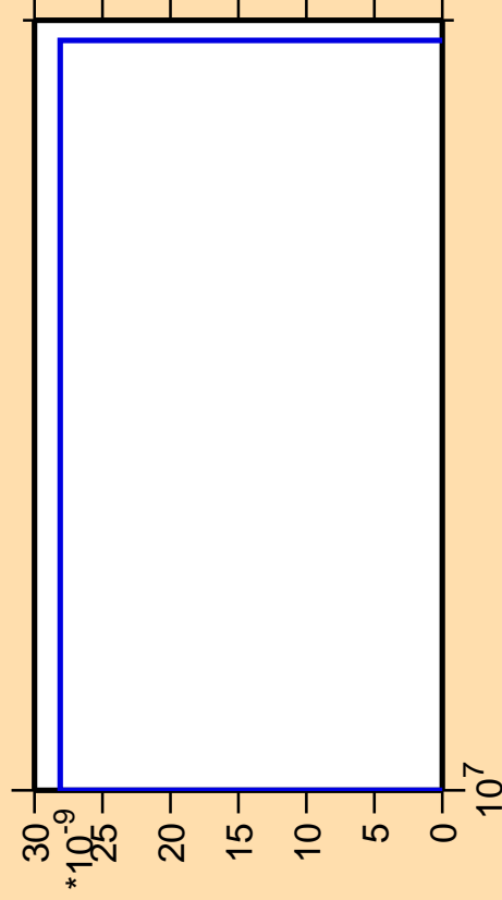
\Delta\sigma/\sigma vs. E for ^{178}\text{Hf} (mt 11)
