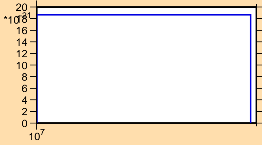
\sigma vs. E for ^{178}\text{Hf} (mt 11)
