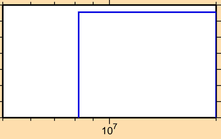
\sigma vs. E for ^{178}\text{Hf}(n,3n\alpha)
