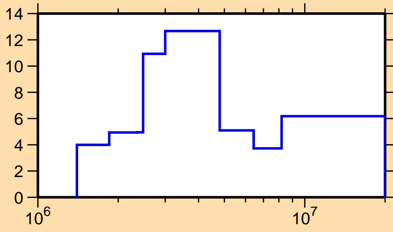
\Delta\sigma/\sigma vs. E for ^{178}\text{Hf}(n,el.)
