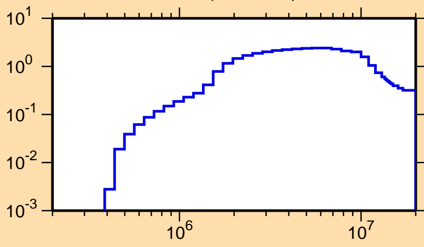
\sigma vs. E for ^{178}\text{Hf}(n,n\text{cont.})
