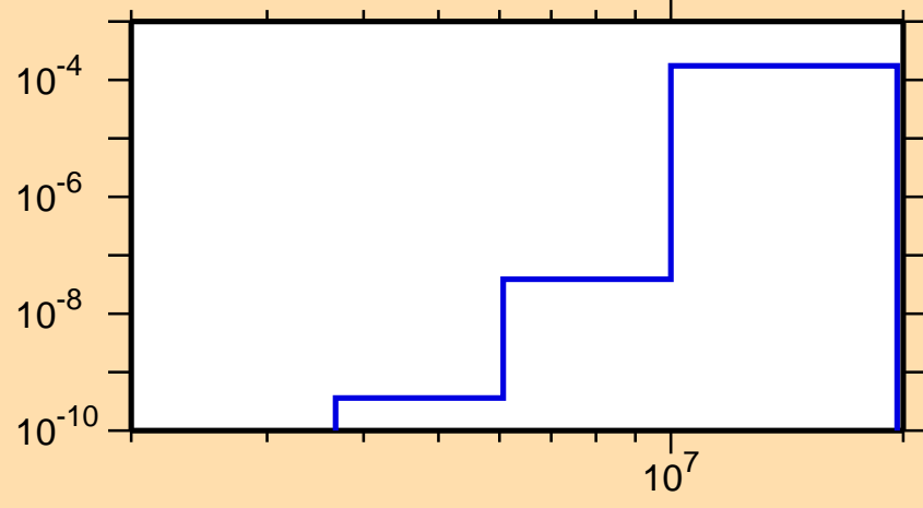
\sigma vs. E for ^{179}\text{Hf}(n,n\alpha)
