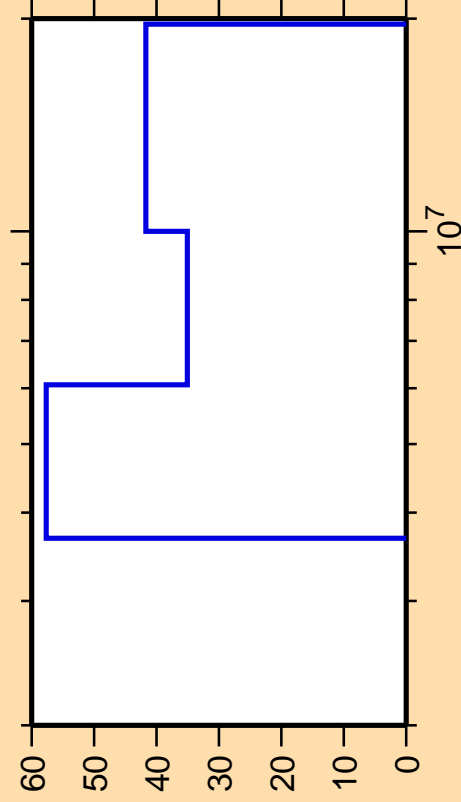
\Delta\sigma/\sigma vs. E for ^{179}\text{Hf}(n,n\alpha)
