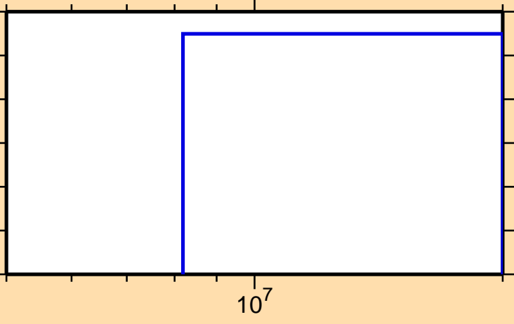
\sigma vs. E for ^{179}\text{Hf}(n,\text{nd})
