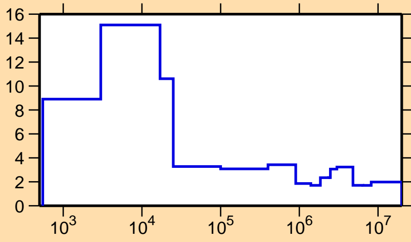
\Delta\sigma/\sigma vs. E for ^{179}\text{Hf}(n,\text{el.})
