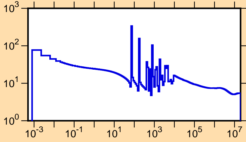
\sigma vs. E for ^{180}\text{Hf}(n,\text{tot.})
