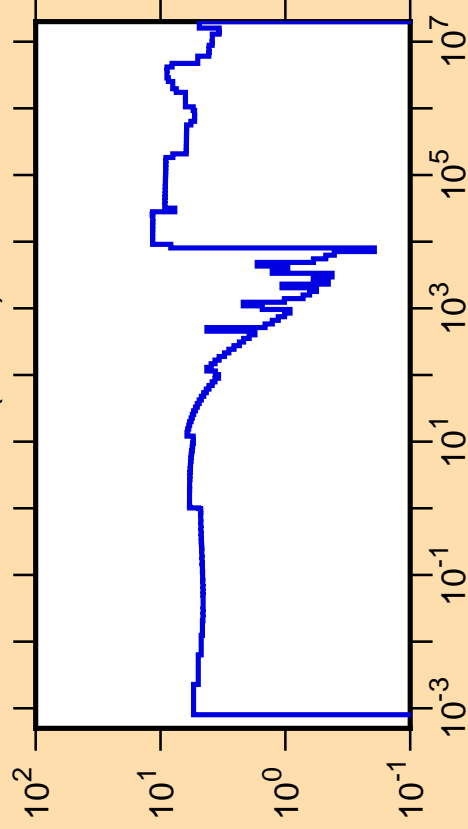
\Delta\sigma/\sigma vs. E for ^{180}\text{Hf}(n,\text{tot.})
