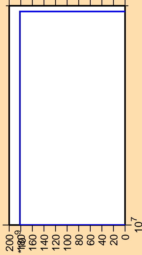
\Delta\sigma/\sigma vs. E for ^{180}\text{Hf} (mt 11)
