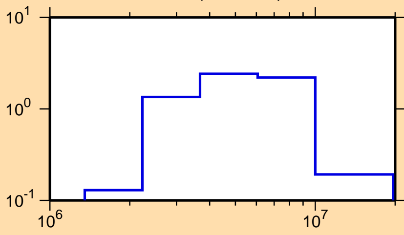
\sigma vs. E for ^{180}\text{Hf}(n,n\text{cont.})
