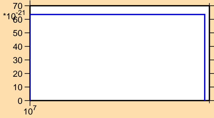
\sigma vs. E for ^{180}\text{Hf} (mt 11)
