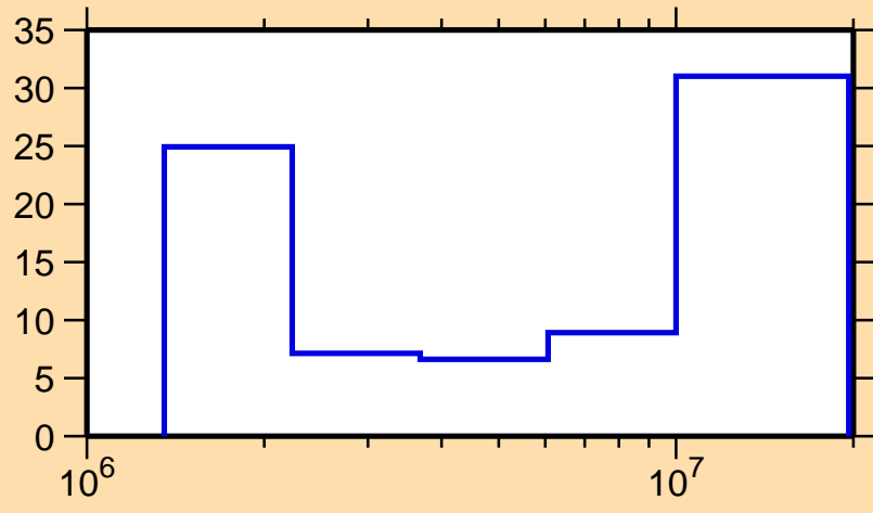
\Delta\sigma/\sigma vs. E for ^{180}\text{Hf}(n,n\text{cont.})
