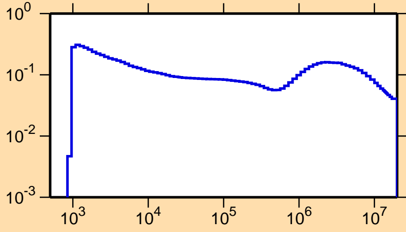
\sigma vs. E for ^{180}\text{Hf}(n,n_3)
