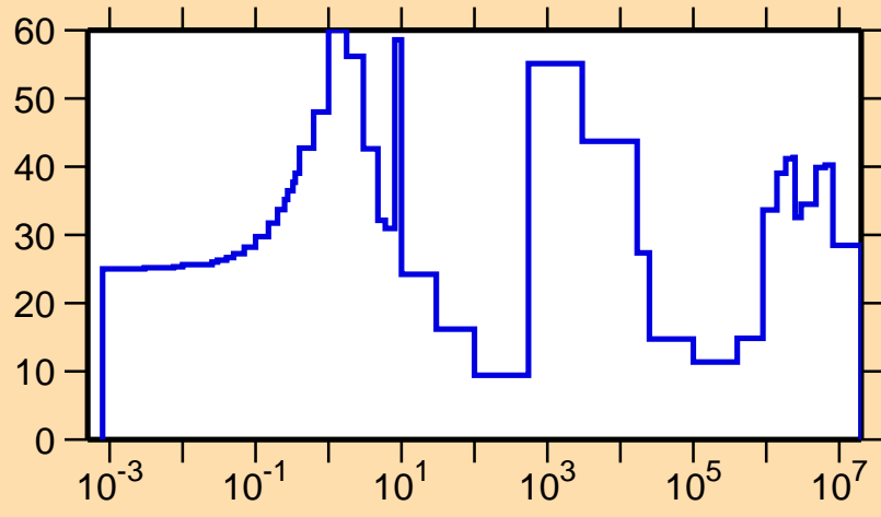
\Delta\sigma/\sigma vs. E for ^{180}\text{Hf}(n,\gamma)
