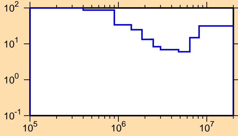
\Delta\sigma/\sigma vs. E for ^{180}\text{Hf}(n,n\text{cont.})
