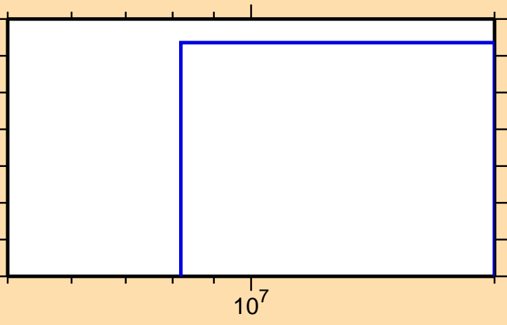
\sigma vs. E for ^{181}\text{Hf}(n,2n\alpha)
