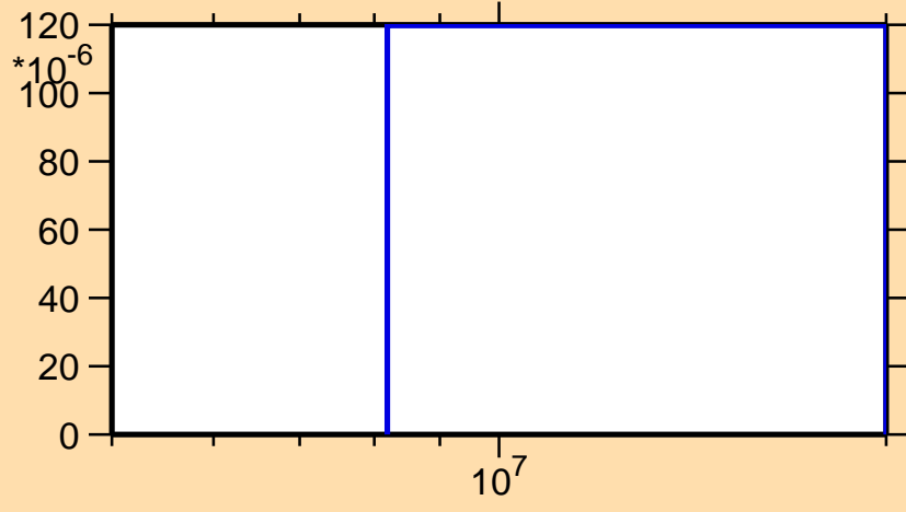
\sigma vs. E for ^{181}\text{Hf}(n,d)
