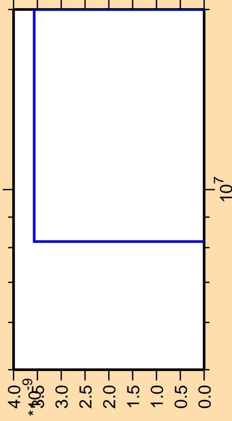
\Delta\sigma/\sigma vs. E for ^{181}\text{Hf}(\text{mt } 11)
