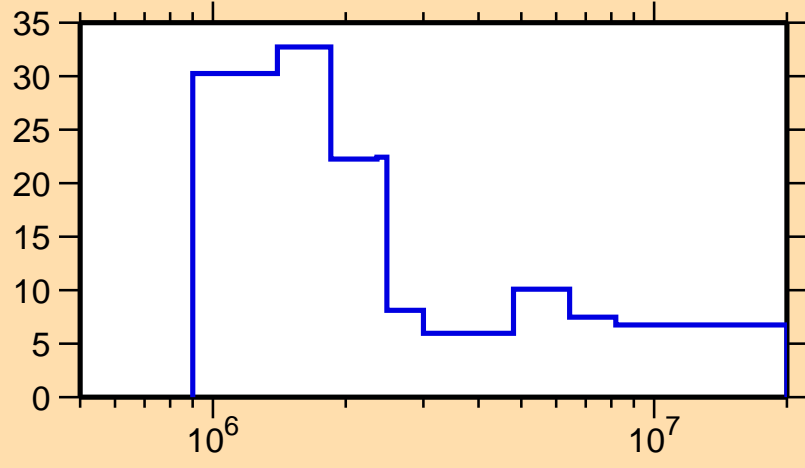
\Delta\sigma/\sigma vs. E for ^{181}\text{Hf}(n,n\text{onel.})
