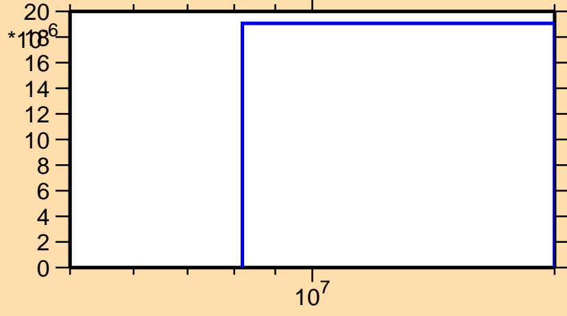
\sigma vs. E for ^{181}\text{Hf}(n,t)
