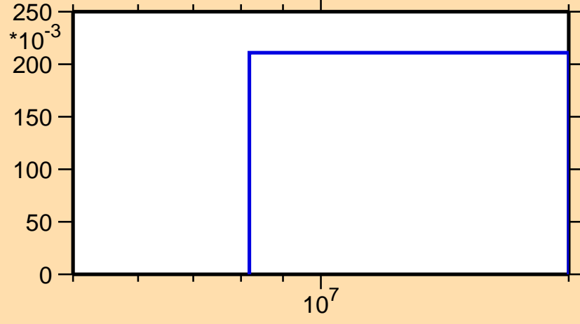
\sigma vs. E for ^{181}\text{Hf}(n,3n)
