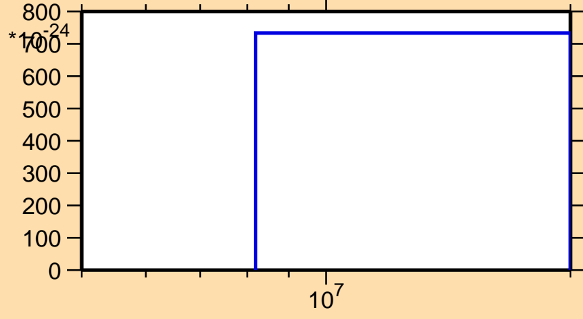
\sigma vs. E for ^{181}\text{Hf}(\text{mt } 11)
