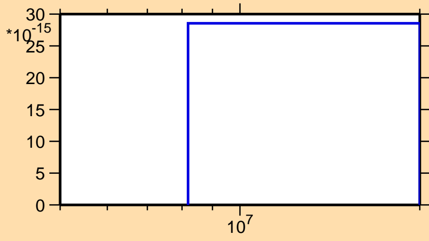
\sigma vs. E for ^{181}\text{Hf}(n,\text{He3})
