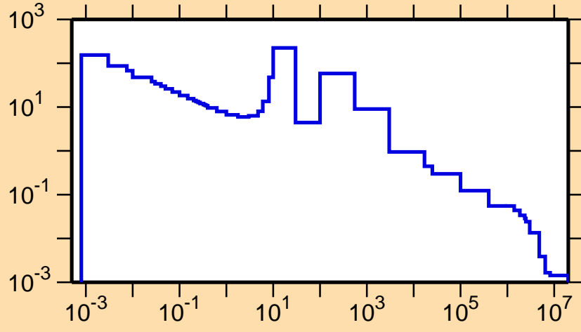
\sigma vs. E for ^{181}\text{Hf}(n,\gamma)
