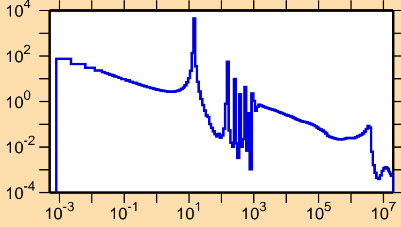
\sigma vs. E for ^{182}\text{Hf}(n,\gamma)
