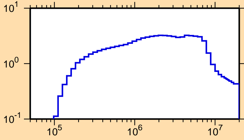
\sigma vs. E for ^{182}\text{Hf}(n,\text{inel.})
