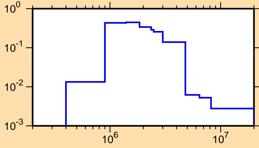
\sigma vs. E for ^{182}\text{Hf}(n,n_4)
