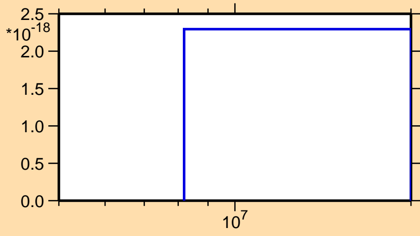
\sigma vs. E for ^{182}\text{Hf}(\text{mt } 11)
