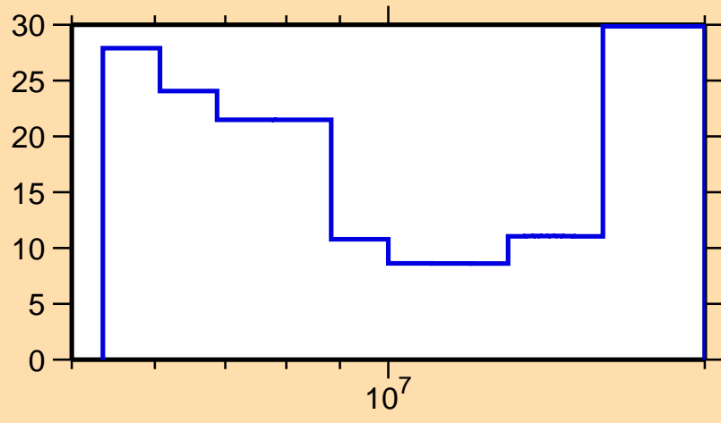
\Delta\sigma/\sigma vs. E for ^{182}\text{Hf}(n,2n)
