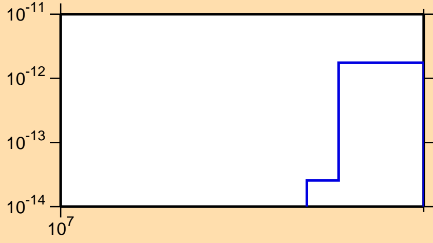
\sigma vs. E for ^{182}\text{Hf}(n,\text{He3})
