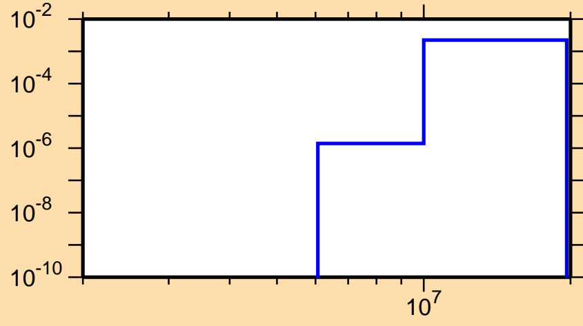
\sigma vs. E for ^{182}\text{Hf}(n,p)
