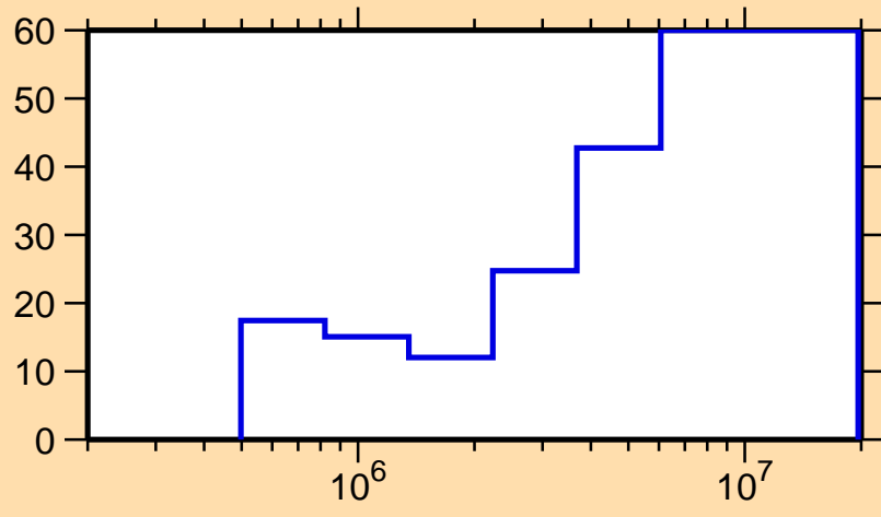
\Delta\sigma/\sigma vs. E for ^{182}\text{Hf}(n,\gamma)
