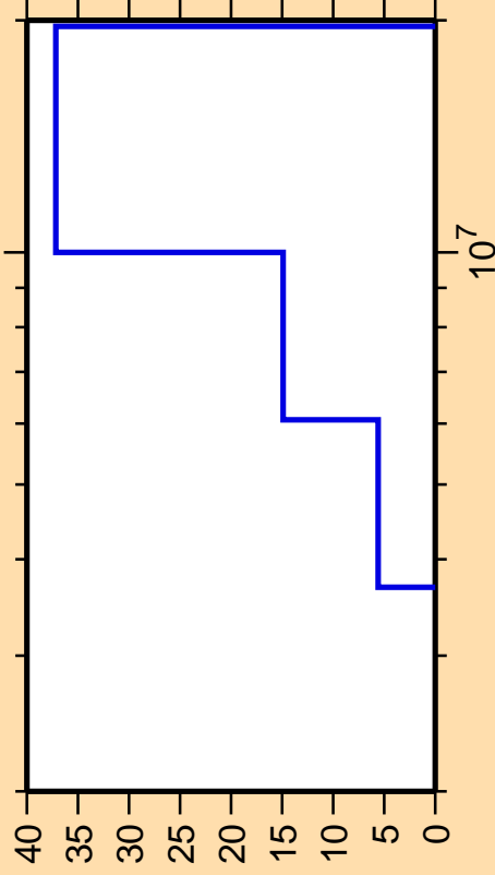
\Delta\sigma/\sigma vs. E for ^{182}\text{Hf}(n,n\text{cont.})
