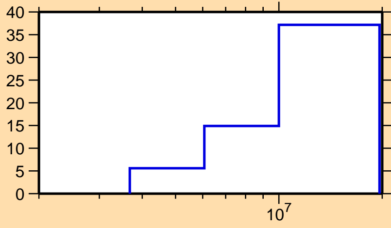
\Delta\sigma/\sigma vs. E for ^{182}\text{Hf}(n,n\text{cont.})
